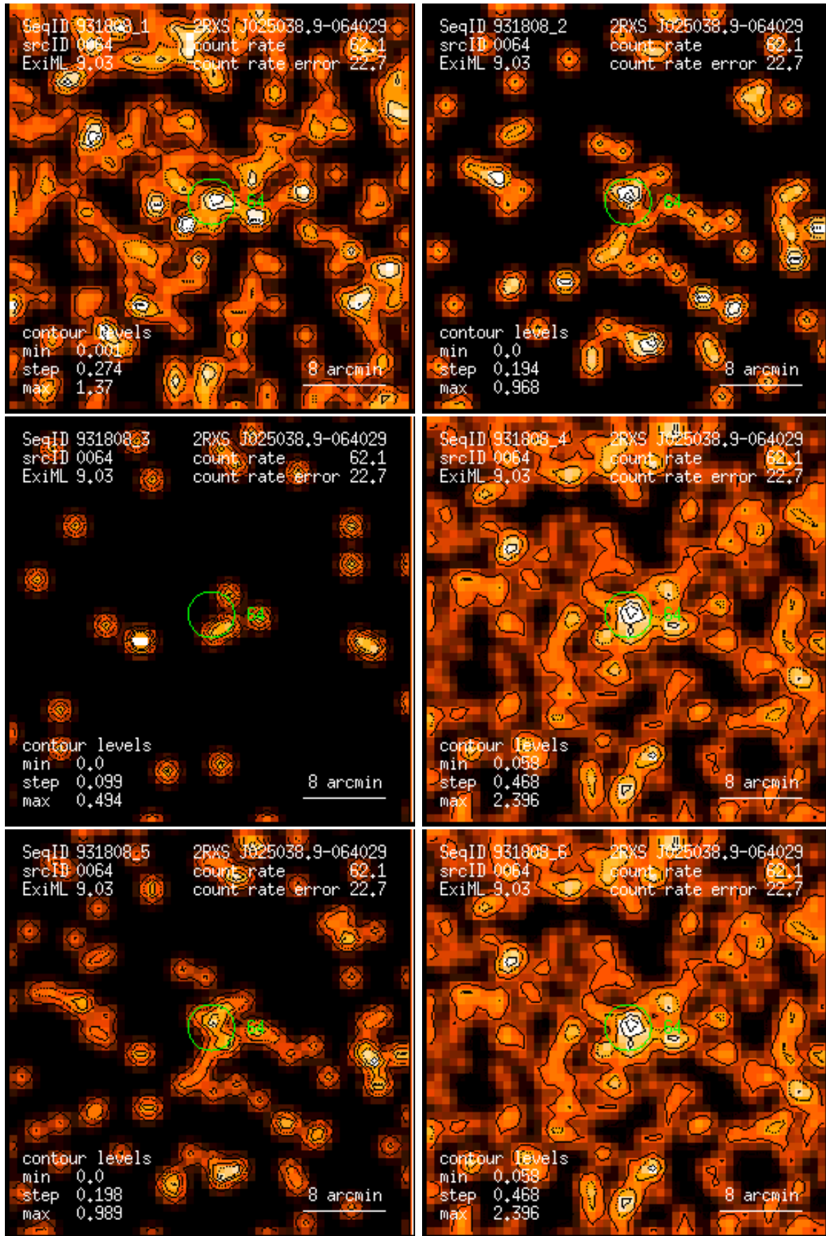
Figure 64: RASS 931808: detection 0064: band rate images, Gaussian filter: (1) PSPC channels 11 – 41, (2) 52 – 90, (3) 91 – 201, (4) 11 – 235, (5) 52 – 201, (6) 11 – 201. Broad band rates in counts/ks. Band rate contour levels in counts/ks/arcmin 2 .
