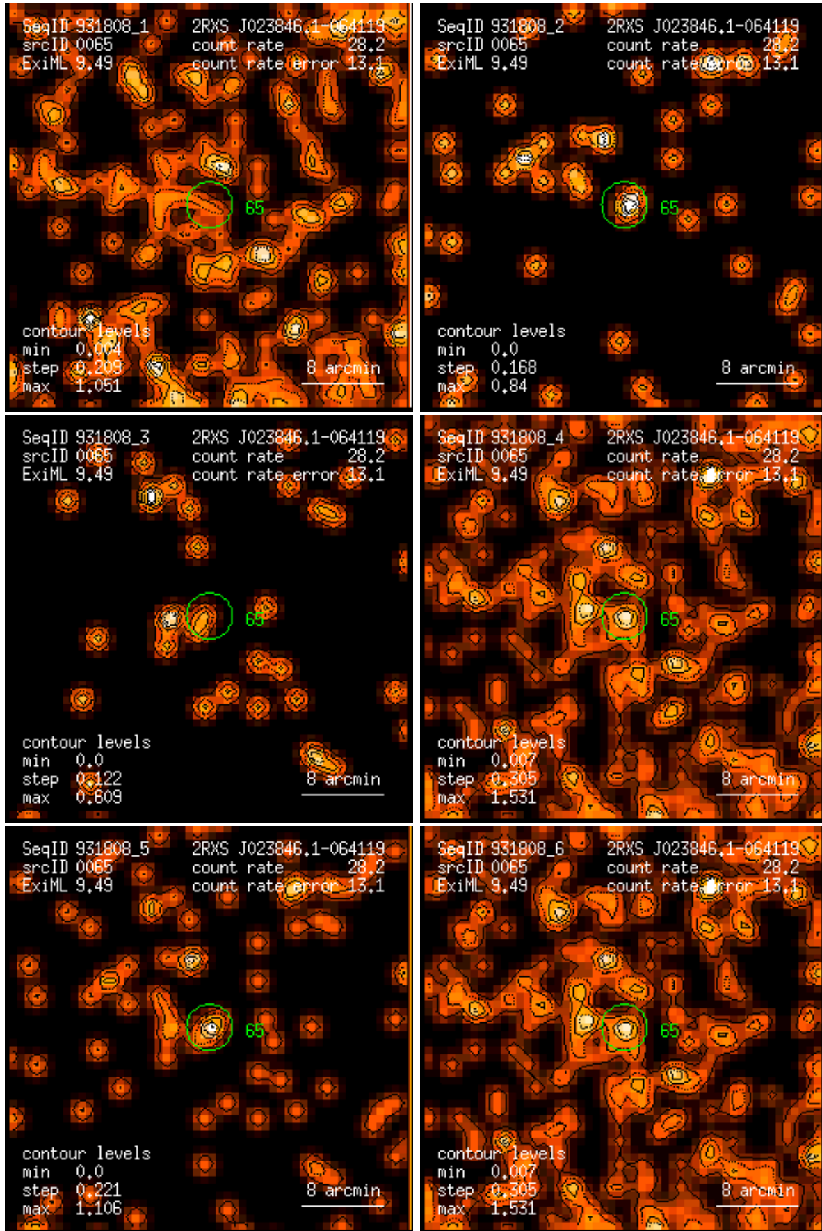
Figure 65: RASS 931808: detection 0065: band rate images, Gaussian filter: (1) PSPC channels 11 – 41, (2) 52 – 90, (3) 91 – 201, (4) 11 – 235, (5) 52 – 201, (6) 11 – 201. Broad band rates in counts/ks. Band rate contour levels in counts/ks/arcmin 2 .
