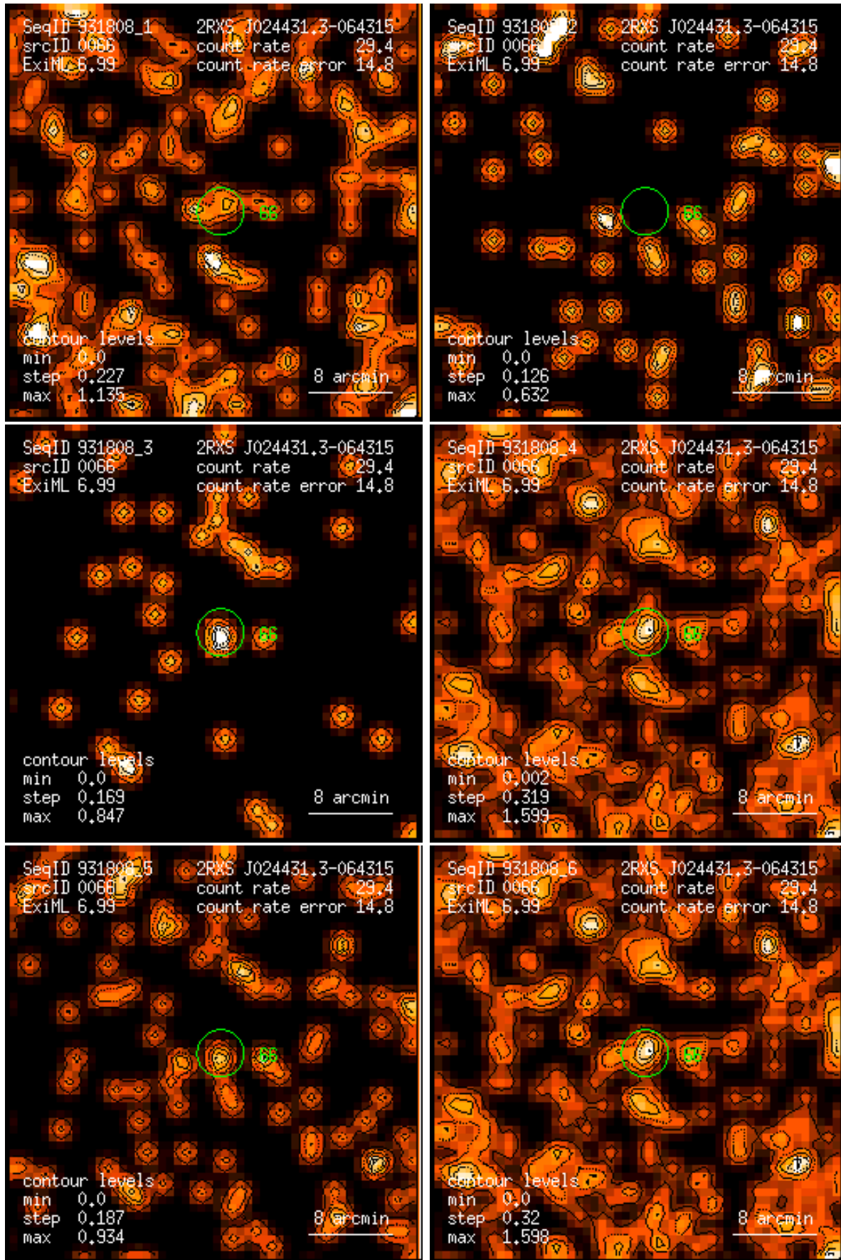
Figure 66: RASS 931808: detection 0066: band rate images, Gaussian filter: (1) PSPC channels 11 – 41, (2) 52 – 90, (3) 91 – 201, (4) 11 – 235, (5) 52 – 201, (6) 11 – 201. Broad band rates in counts/ks. Band rate contour levels in counts/ks/arcmin 2 .
