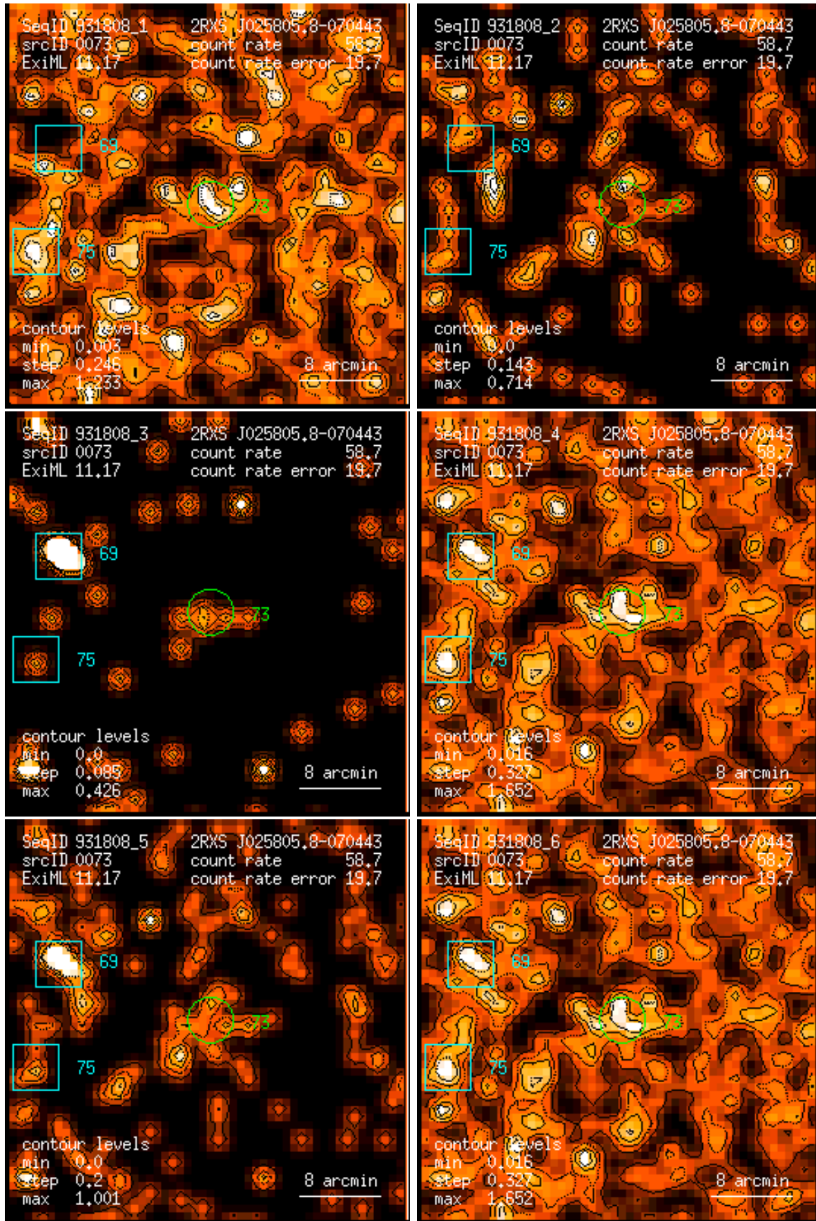
Figure 73: RASS 931808: detection 0073: band rate images, Gaussian filter: (1) PSPC channels 11 – 41, (2) 52 – 90, (3) 91 – 201, (4) 11 – 235, (5) 52 – 201, (6) 11 – 201. Broad band rates in counts/ks. Band rate contour levels in counts/ks/arcmin 2 .
