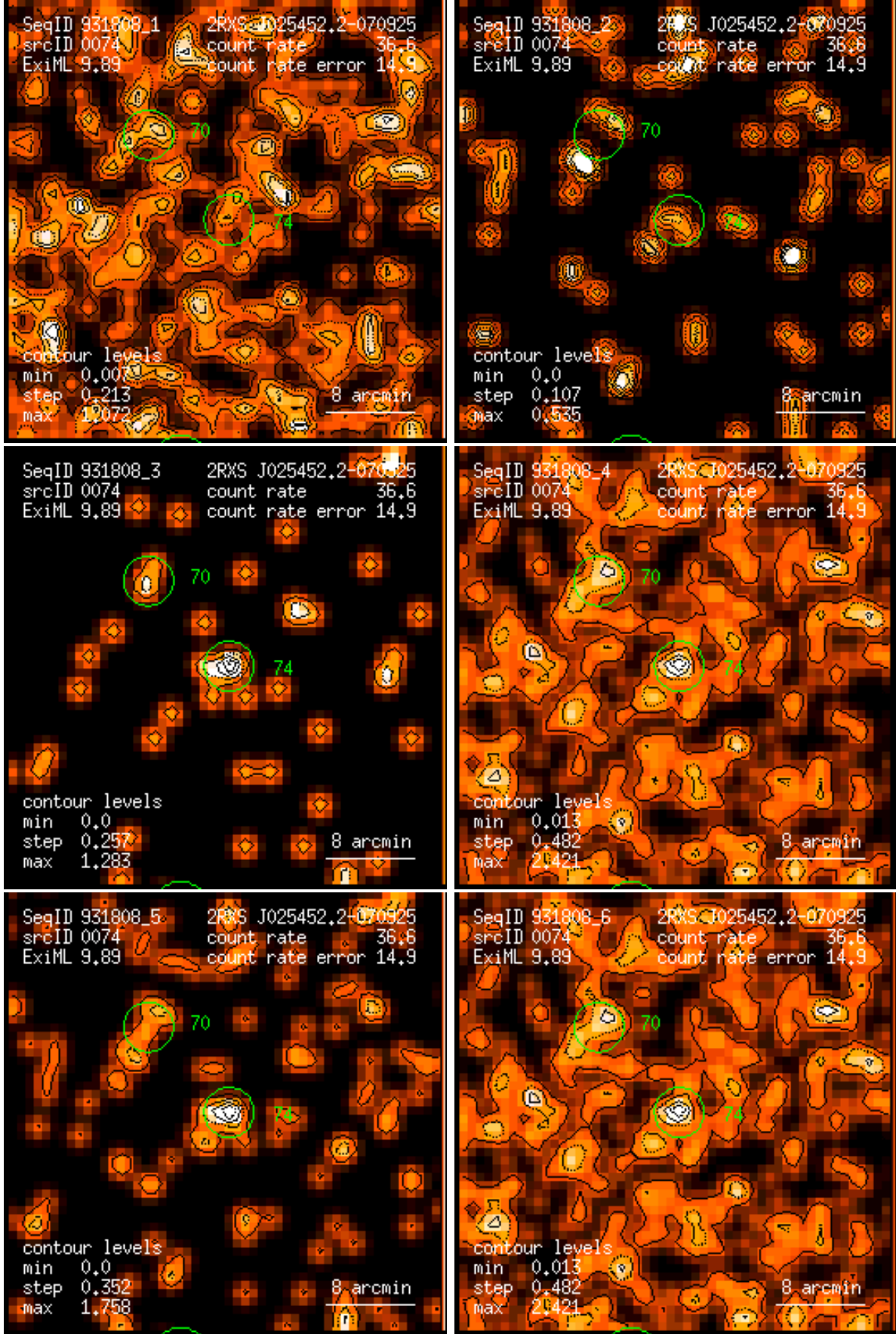
Figure 74: RASS 931808: detection 0074: band rate images, Gaussian filter: (1) PSPC channels 11 – 41, (2) 52 – 90, (3) 91 – 201, (4) 11 – 235, (5) 52 – 201, (6) 11 – 201. Broad band rates in counts/ks. Band rate contour levels in counts/ks/arcmin 2 .
