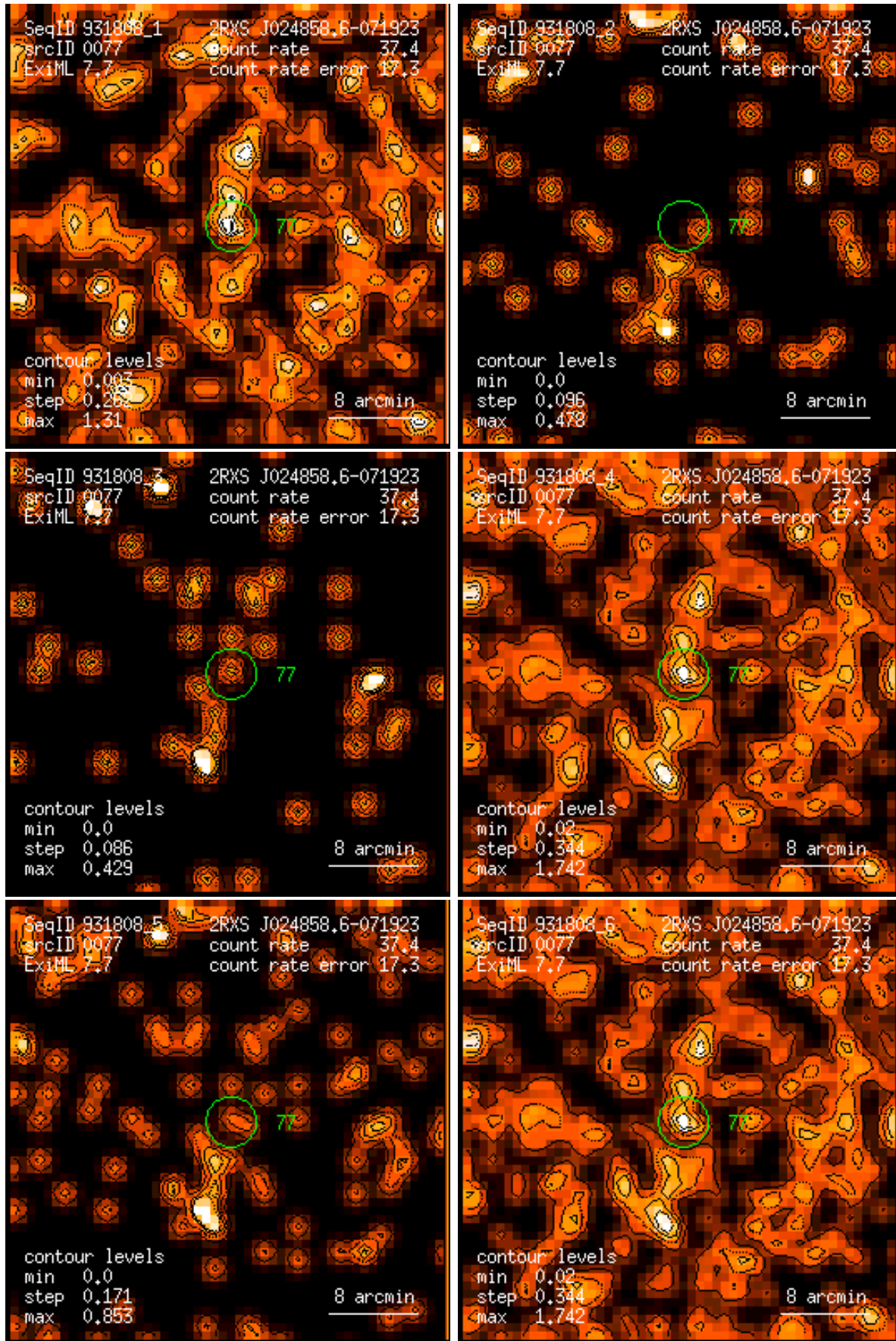
Figure 77: RASS 931808: detection 0077: band rate images, Gaussian filter: (1) PSPC channels 11 – 41, (2) 52 – 90, (3) 91 – 201, (4) 11 – 235, (5) 52 – 201, (6) 11 – 201. Broad band rates in counts/ks. Band rate contour levels in counts/ks/arcmin 2 .
