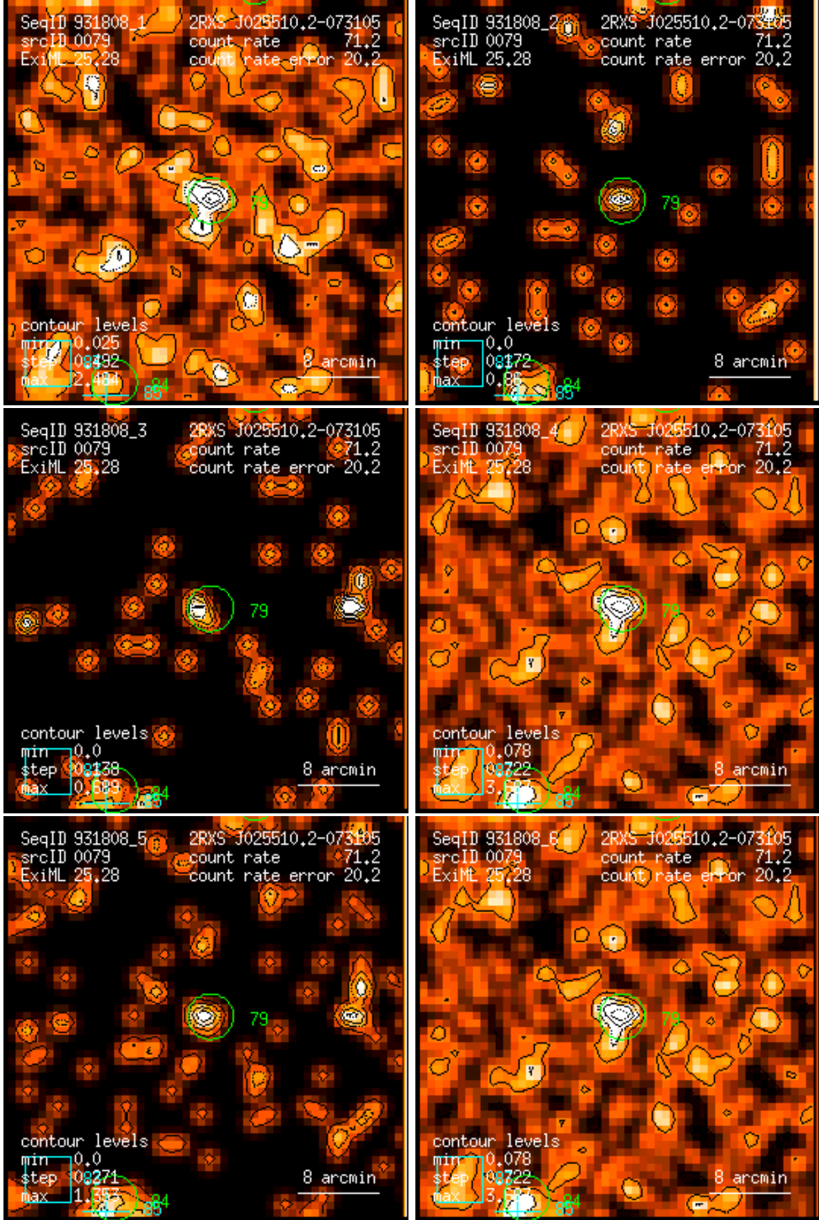
Figure 79: RASS 931808: detection 0079: band rate images, Gaussian filter: (1) PSPC channels 11 – 41, (2) 52 – 90, (3) 91 – 201, (4) 11 – 235, (5) 52 – 201, (6) 11 – 201. Broad band rates in counts/ks. Band rate contour levels in counts/ks/arcmin 2 .
