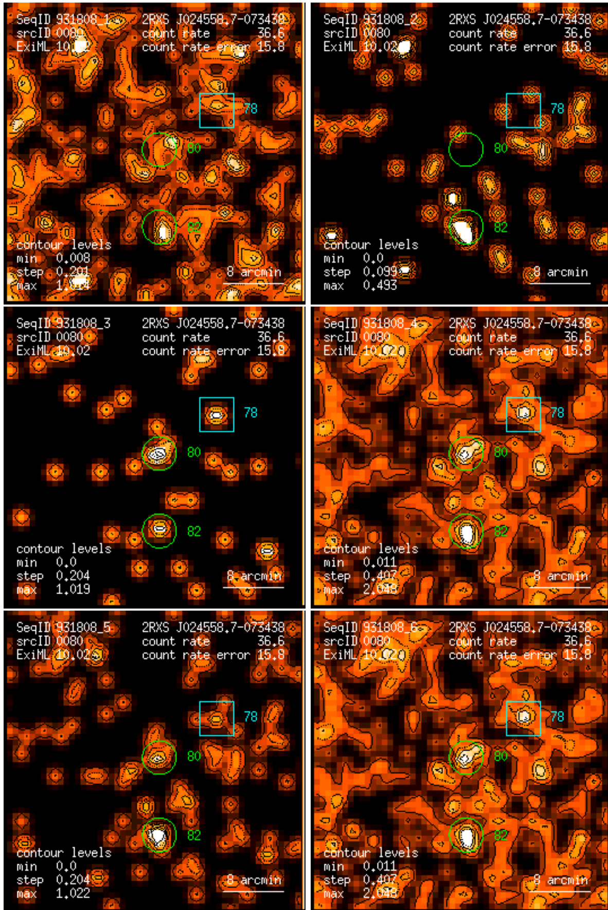
Figure 80: RASS 931808: detection 0080: band rate images, Gaussian filter: (1) PSPC channels 11 – 41, (2) 52 – 90, (3) 91 – 201, (4) 11 – 235, (5) 52 – 201, (6) 11 – 201. Broad band rates in counts/ks. Band rate contour levels in counts/ks/arcmin 2 .
