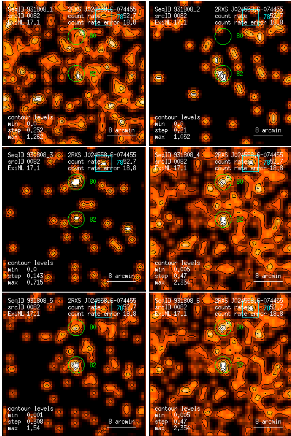
Figure 82: RASS 931808: detection 0082: band rate images, Gaussian filter: (1) PSPC channels 11 – 41, (2) 52 – 90, (3) 91 – 201, (4) 11 – 235, (5) 52 – 201, (6) 11 – 201. Broad band rates in counts/ks. Band rate contour levels in counts/ks/arcmin 2 .
