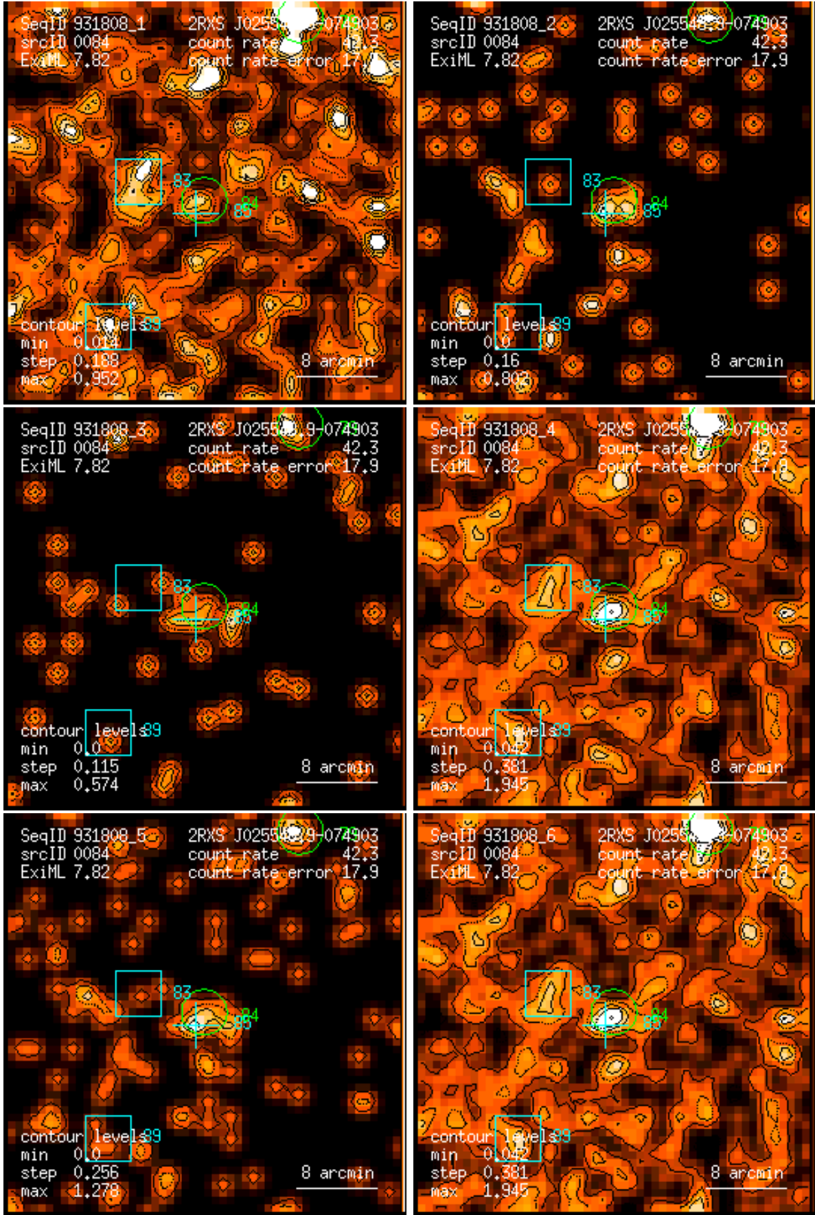
Figure 84: RASS 931808: detection 0084: band rate images, Gaussian filter: (1) PSPC channels 11 – 41, (2) 52 – 90, (3) 91 – 201, (4) 11 – 235, (5) 52 – 201, (6) 11 – 201. Broad band rates in counts/ks. Band rate contour levels in counts/ks/arcmin 2 .
