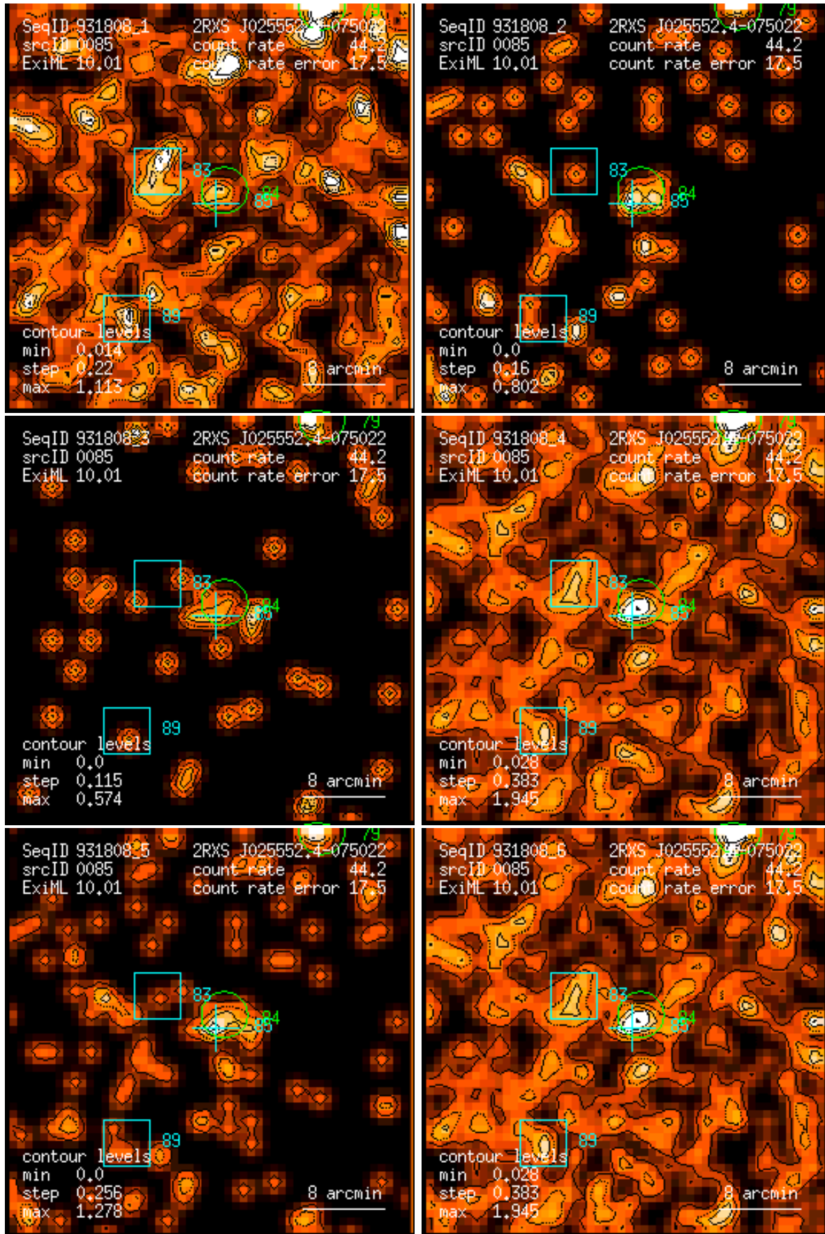
Figure 85: RASS 931808: detection 0085: band rate images, Gaussian filter: (1) PSPC channels 11 – 41, (2) 52 – 90, (3) 91 – 201, (4) 11 – 235, (5) 52 – 201, (6) 11 – 201. Broad band rates in counts/ks. Band rate contour levels in counts/ks/arcmin 2 .
