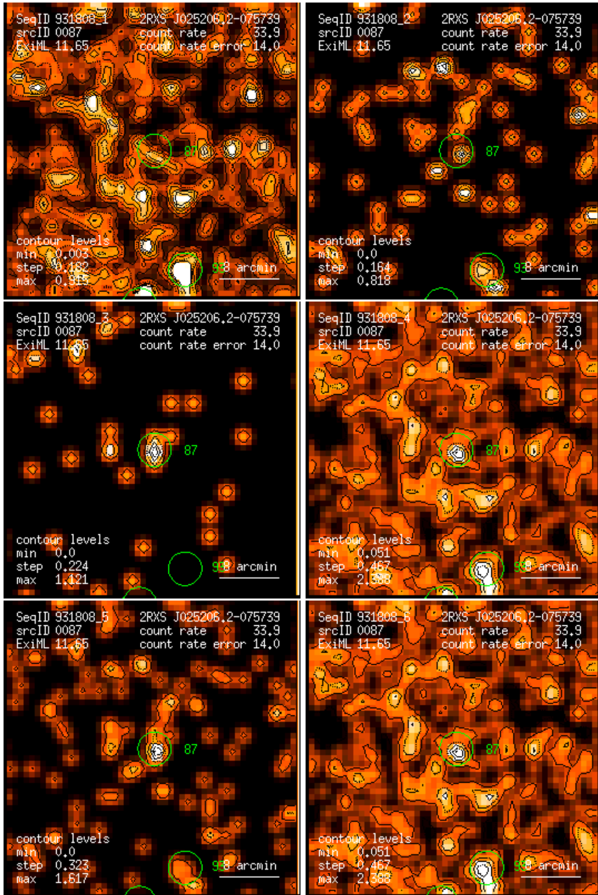
Figure 87: RASS 931808: detection 0087: band rate images, Gaussian filter: (1) PSPC channels 11 – 41, (2) 52 – 90, (3) 91 – 201, (4) 11 – 235, (5) 52 – 201, (6) 11 – 201. Broad band rates in counts/ks. Band rate contour levels in counts/ks/arcmin 2 .
