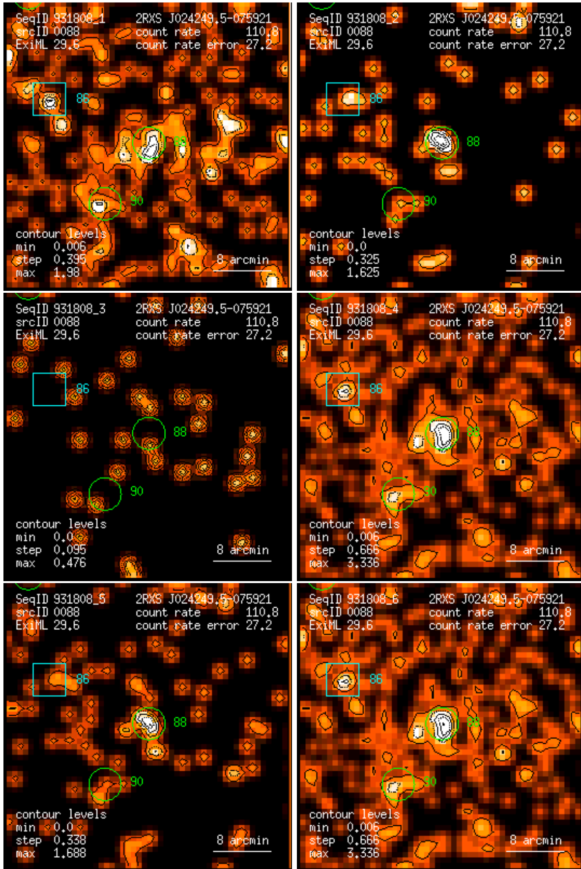
Figure 88: RASS 931808: detection 0088: band rate images, Gaussian filter: (1) PSPC channels 11 – 41, (2) 52 – 90, (3) 91 – 201, (4) 11 – 235, (5) 52 – 201, (6) 11 – 201. Broad band rates in counts/ks. Band rate contour levels in counts/ks/arcmin 2 .
