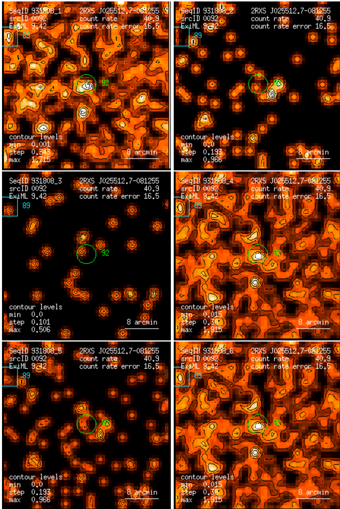
Figure 92: RASS 931808: detection 0092: band rate images, Gaussian filter: (1) PSPC channels 11 – 41, (2) 52 – 90, (3) 91 – 201, (4) 11 – 235, (5) 52 – 201, (6) 11 – 201. Broad band rates in counts/ks. Band rate contour levels in counts/ks/arcmin 2 .
