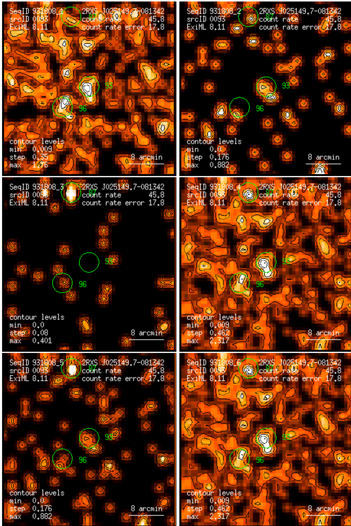
Figure 93: RASS 931808: detection 0093: band rate images, Gaussian filter: (1) PSPC channels 11 – 41, (2) 52 – 90, (3) 91 – 201, (4) 11 – 235, (5) 52 – 201, (6) 11 – 201. Broad band rates in counts/ks. Band rate contour levels in counts/ks/arcmin 2 .
