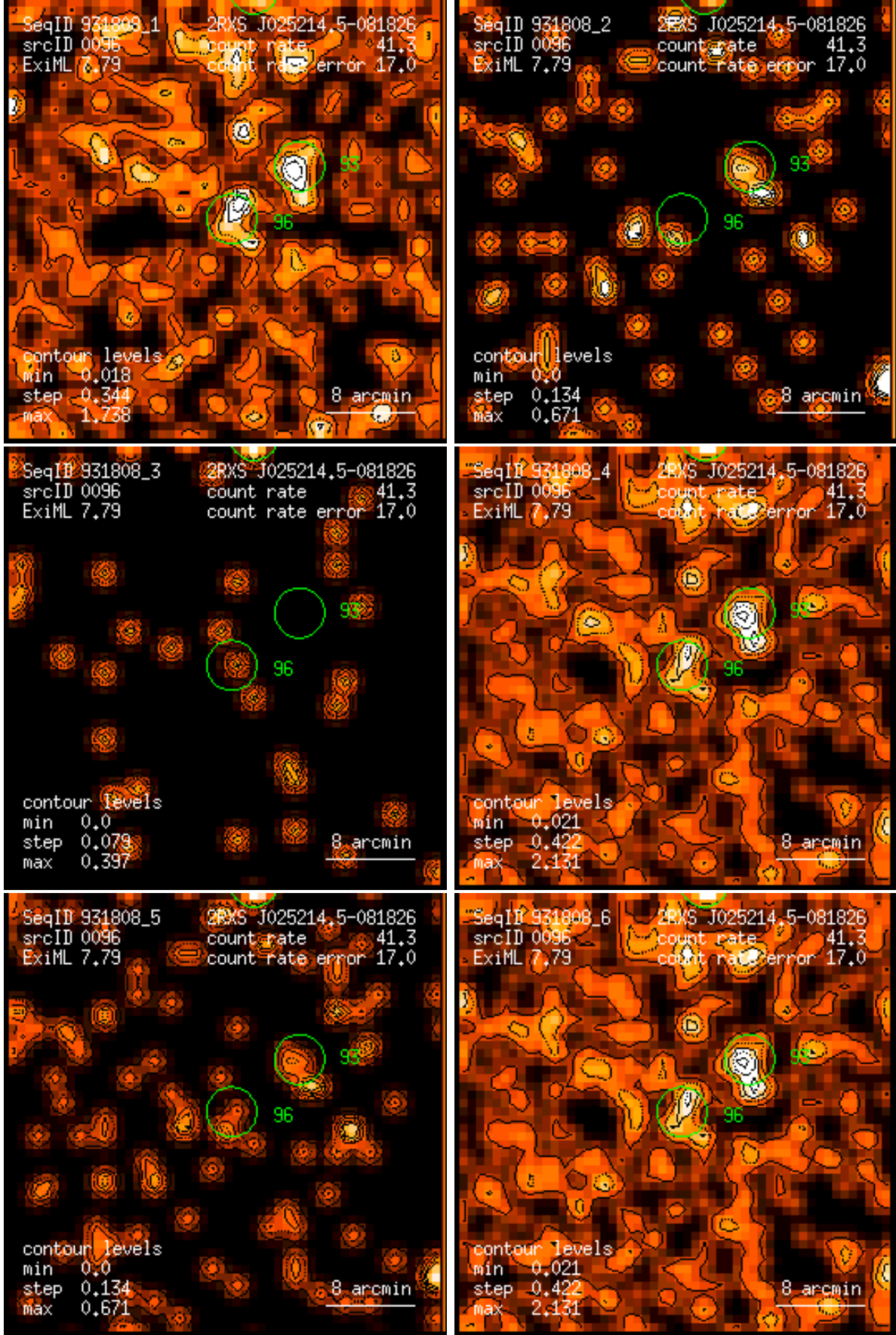
Figure 96: RASS 931808: detection 0096: band rate images, Gaussian filter: (1) PSPC channels 11 – 41, (2) 52 – 90, (3) 91 – 201, (4) 11 – 235, (5) 52 – 201, (6) 11 – 201. Broad band rates in counts/ks. Band rate contour levels in counts/ks/arcmin 2 .
