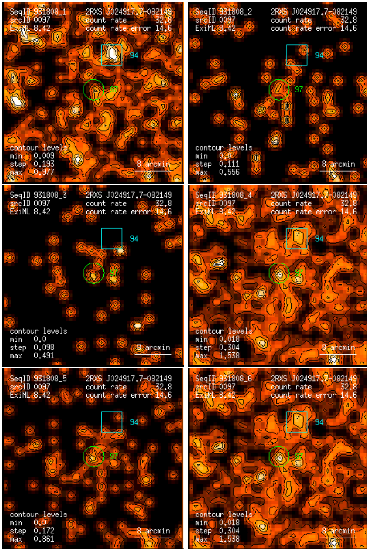
Figure 97: RASS 931808: detection 0097: band rate images, Gaussian filter: (1) PSPC channels 11 – 41, (2) 52 – 90, (3) 91 – 201, (4) 11 – 235, (5) 52 – 201, (6) 11 – 201. Broad band rates in counts/ks. Band rate contour levels in counts/ks/arcmin 2 .
