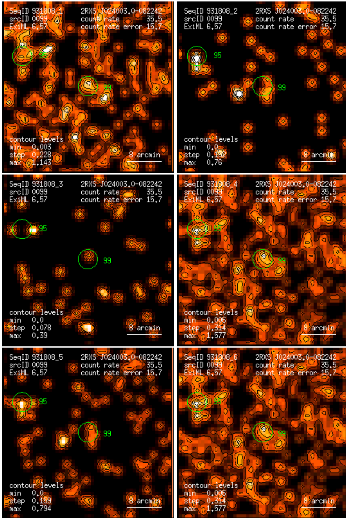
Figure 99: RASS 931808: detection 0099: band rate images, Gaussian filter: (1) PSPC channels 11 – 41, (2) 52 – 90, (3) 91 – 201, (4) 11 – 235, (5) 52 – 201, (6) 11 – 201. Broad band rates in counts/ks. Band rate contour levels in counts/ks/arcmin 2 .
