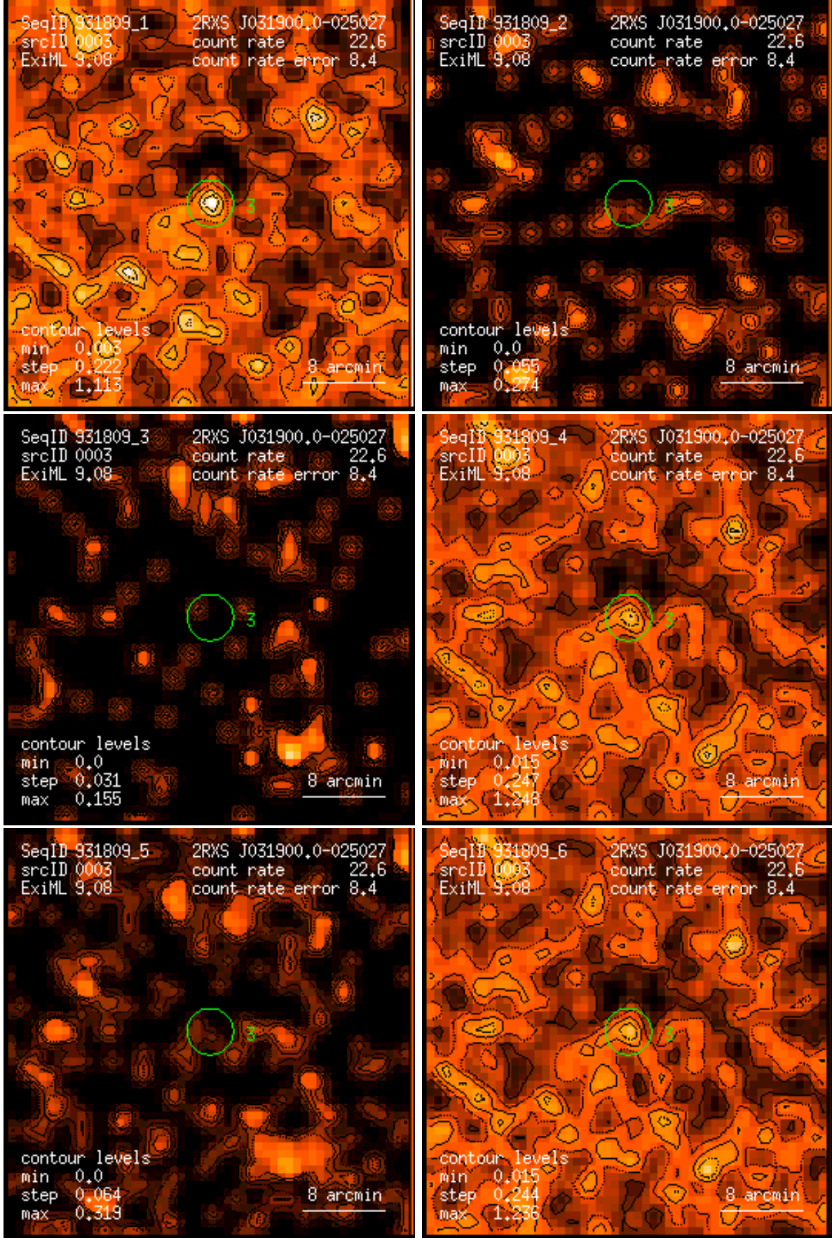
Figure 3: RASS 931809: detection 0003: band rate images, Gaussian filter: (1) PSPC channels 11 – 41, (2) 52 – 90, (3) 91 – 201, (4) 11 – 235, (5) 52 – 201, (6) 11 – 201. Broad band rates in counts/ks. Band rate contour levels in counts/ks/arcmin 2 .
