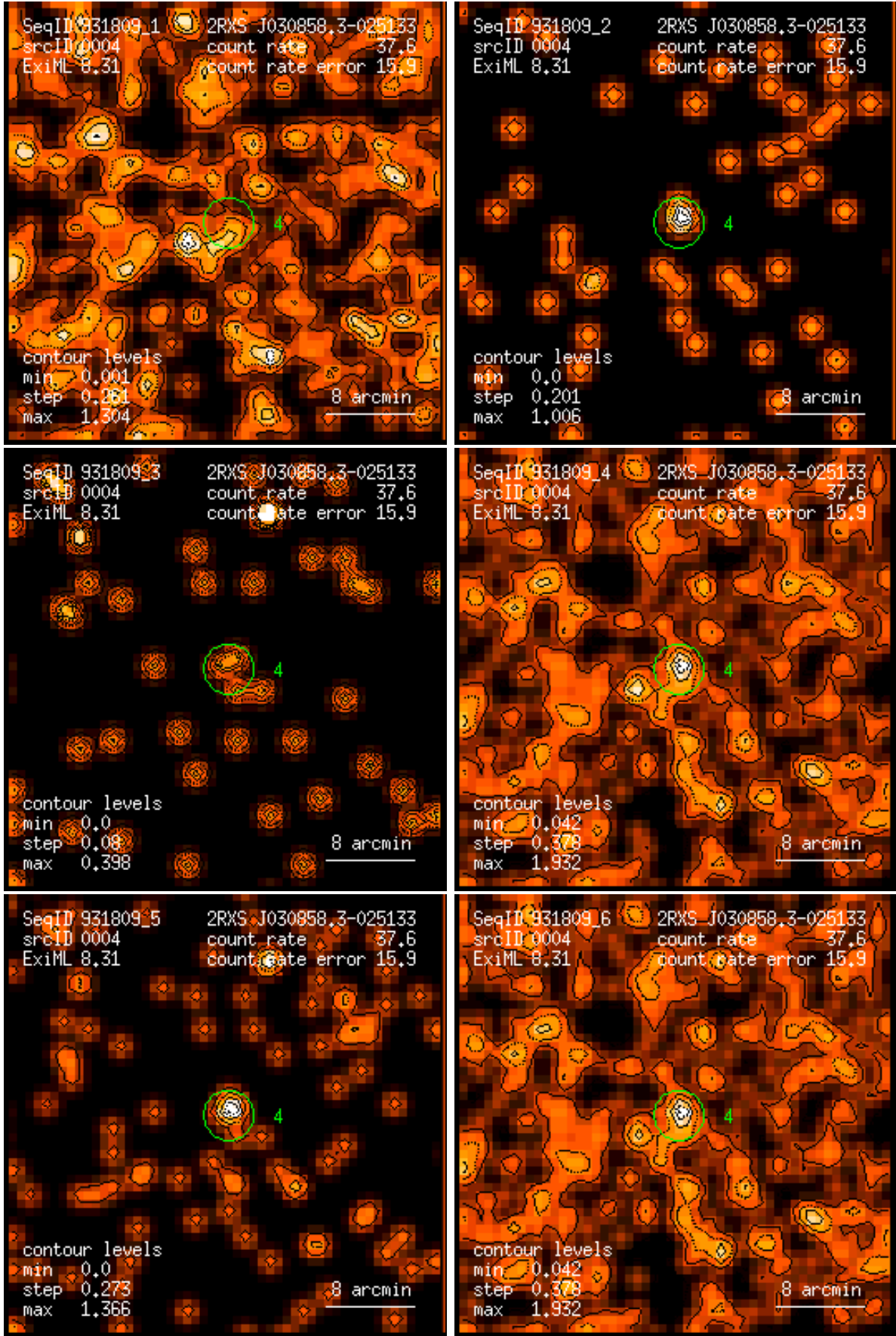
Figure 4: RASS 931809: detection 0004: band rate images, Gaussian filter: (1) PSPC channels 11 – 41, (2) 52 – 90, (3) 91 – 201, (4) 11 – 235, (5) 52 – 201, (6) 11 – 201. Broad band rates in counts/ks. Band rate contour levels in counts/ks/arcmin 2 .
