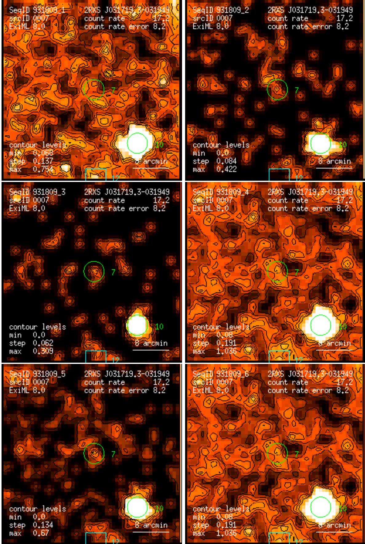
Figure 7: RASS 931809: detection 0007: band rate images, Gaussian filter: (1) PSPC channels 11 – 41, (2) 52 – 90, (3) 91 – 201, (4) 11 – 235, (5) 52 – 201, (6) 11 – 201. Broad band rates in counts/ks. Band rate contour levels in counts/ks/arcmin 2 .
