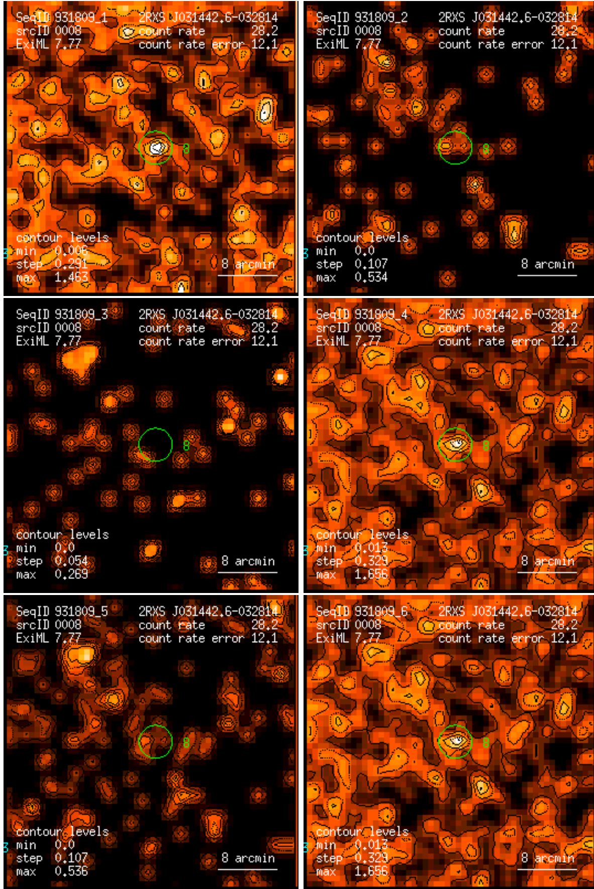
Figure 8: RASS 931809: detection 0008: band rate images, Gaussian filter: (1) PSPC channels 11 – 41, (2) 52 – 90, (3) 91 – 201, (4) 11 – 235, (5) 52 – 201, (6) 11 – 201. Broad band rates in counts/ks. Band rate contour levels in counts/ks/arcmin 2 .
