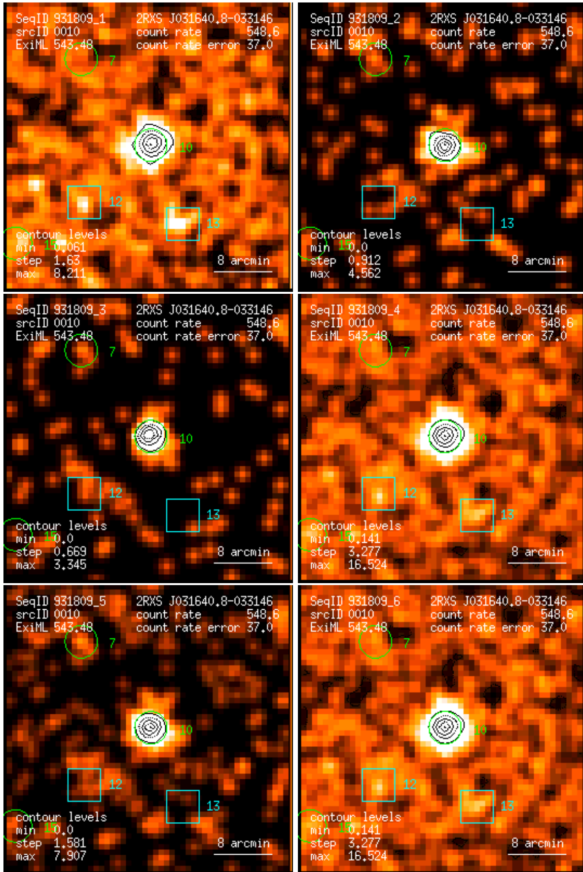
Figure 10: RASS 931809: detection 0010: band rate images, Gaussian filter: (1) PSPC channels 11 – 41, (2) 52 – 90, (3) 91 – 201, (4) 11 – 235, (5) 52 – 201, (6) 11 – 201. Broad band rates in counts/ks. Band rate contour levels in counts/ks/arcmin 2 .
