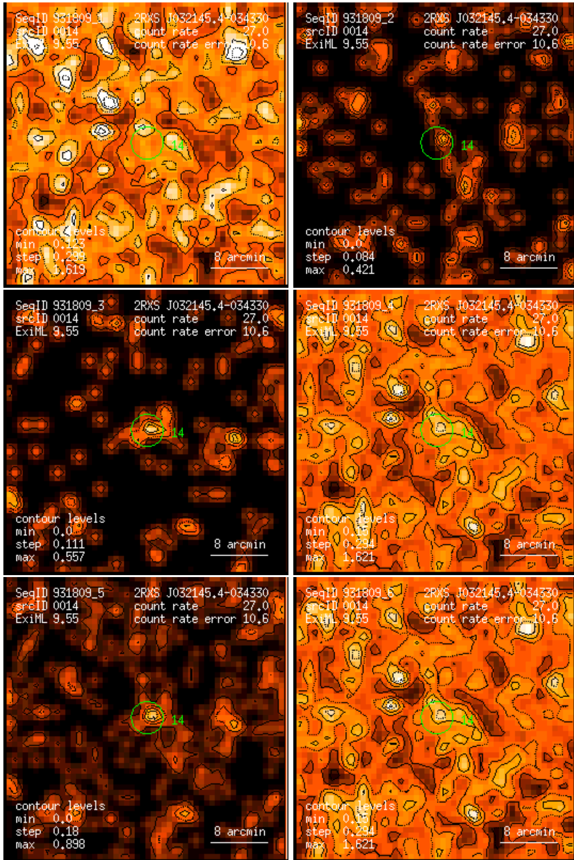
Figure 14: RASS 931809: detection 0014: band rate images, Gaussian filter: (1) PSPC channels 11 – 41, (2) 52 – 90, (3) 91 – 201, (4) 11 – 235, (5) 52 – 201, (6) 11 – 201. Broad band rates in counts/ks. Band rate contour levels in counts/ks/arcmin 2 .
