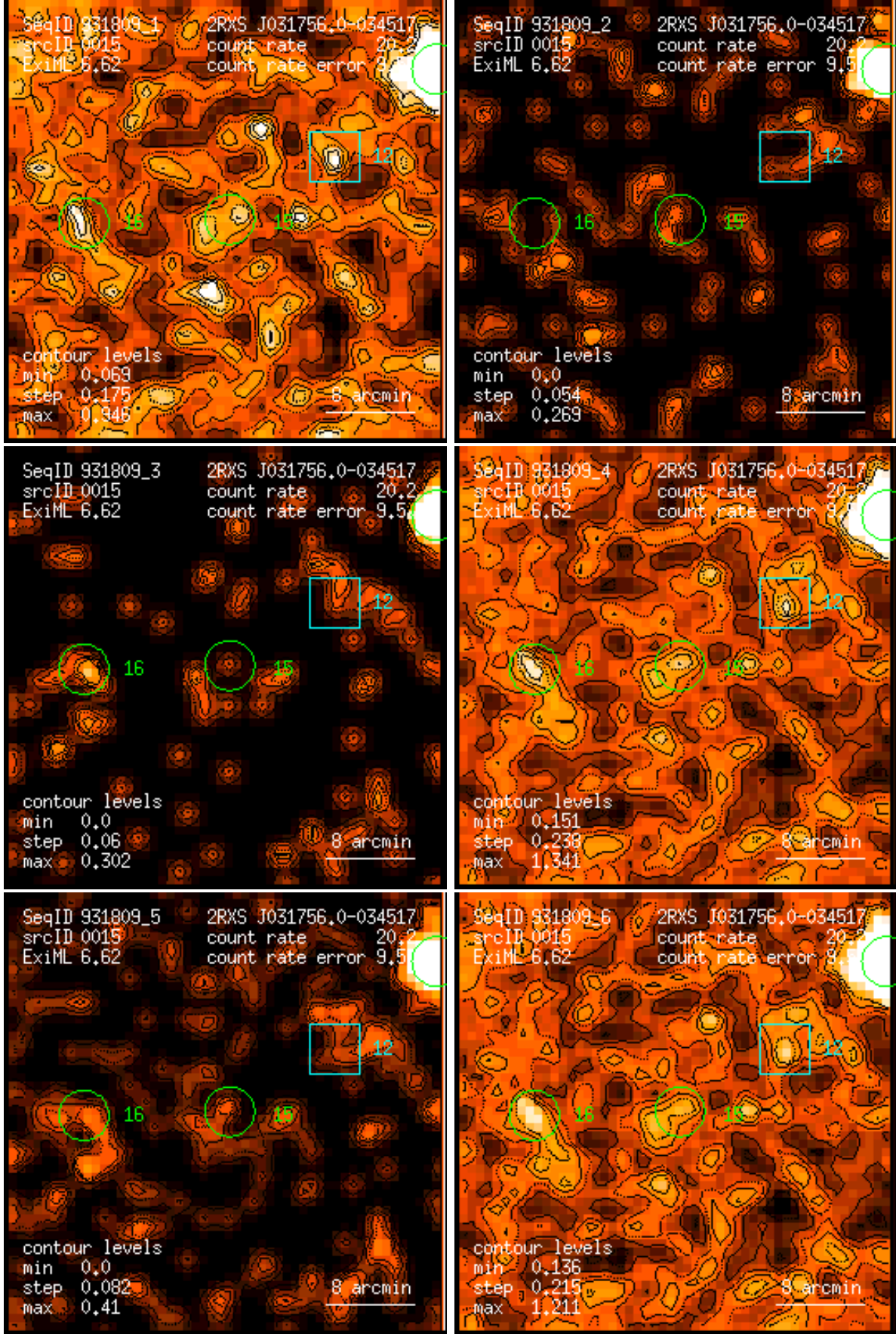
Figure 15: RASS 931809: detection 0015: band rate images, Gaussian filter: (1) PSPC channels 11 – 41, (2) 52 – 90, (3) 91 – 201, (4) 11 – 235, (5) 52 – 201, (6) 11 – 201. Broad band rates in counts/ks. Band rate contour levels in counts/ks/arcmin 2 .
