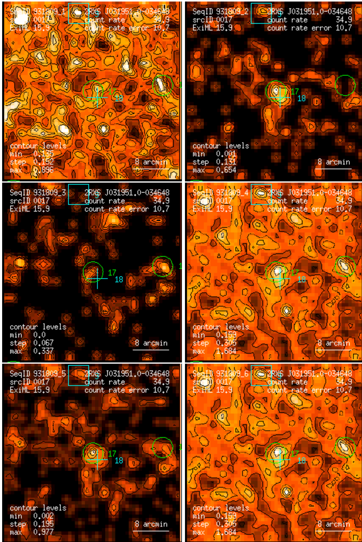
Figure 17: RASS 931809: detection 0017: band rate images, Gaussian filter: (1) PSPC channels 11 – 41, (2) 52 – 90, (3) 91 – 201, (4) 11 – 235, (5) 52 – 201, (6) 11 – 201. Broad band rates in counts/ks. Band rate contour levels in counts/ks/arcmin 2 .
