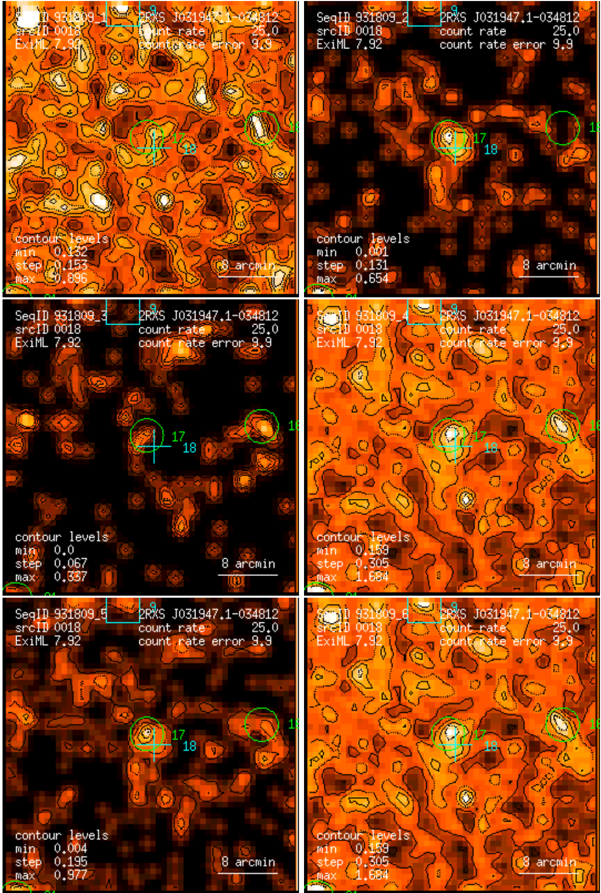
Figure 18: RASS 931809: detection 0018: band rate images, Gaussian filter: (1) PSPC channels 11 – 41, (2) 52 – 90, (3) 91 – 201, (4) 11 – 235, (5) 52 – 201, (6) 11 – 201. Broad band rates in counts/ks. Band rate contour levels in counts/ks/arcmin 2 .
