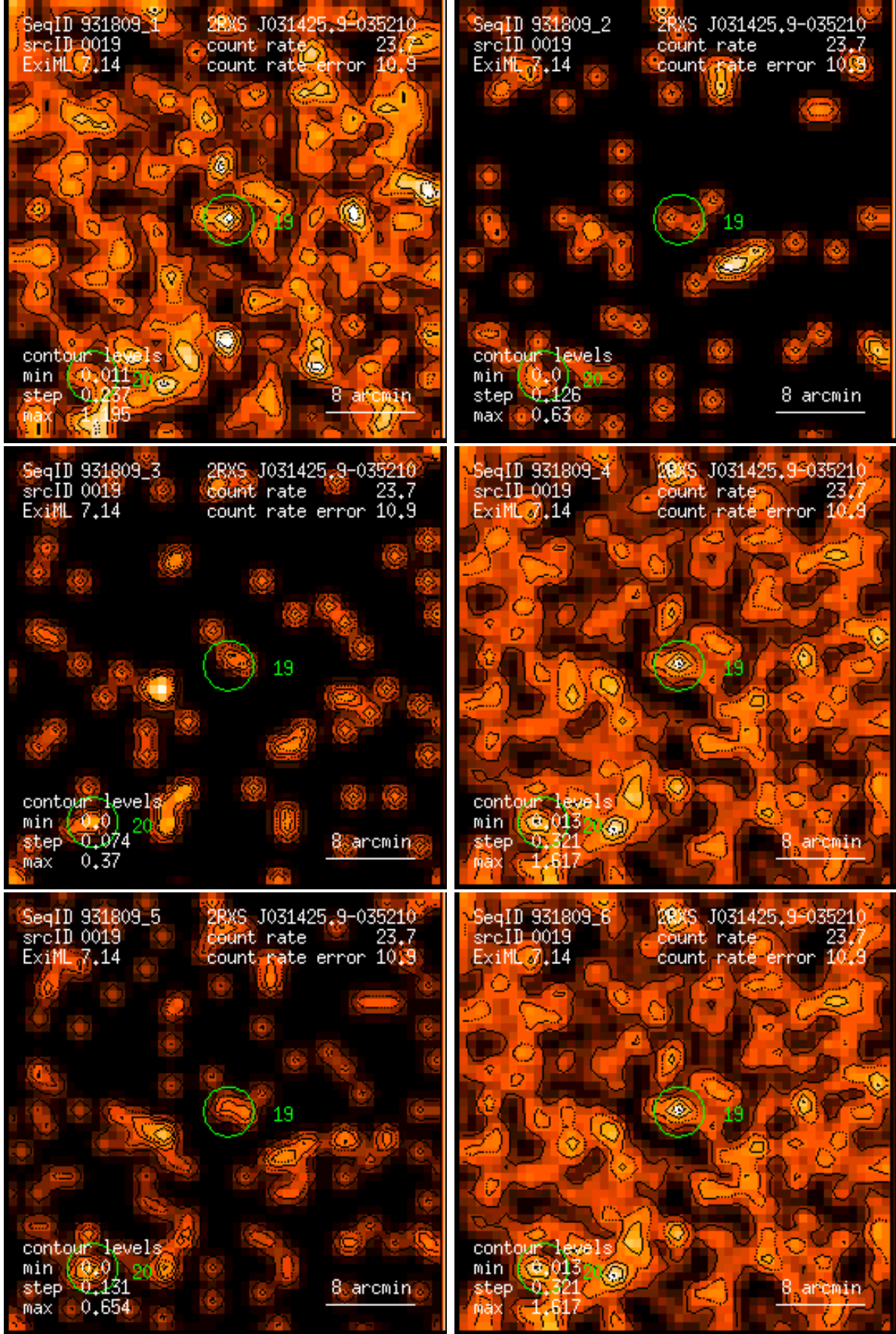
Figure 19: RASS 931809: detection 0019: band rate images, Gaussian filter: (1) PSPC channels 11 – 41, (2) 52 – 90, (3) 91 – 201, (4) 11 – 235, (5) 52 – 201, (6) 11 – 201. Broad band rates in counts/ks. Band rate contour levels in counts/ks/arcmin 2 .
