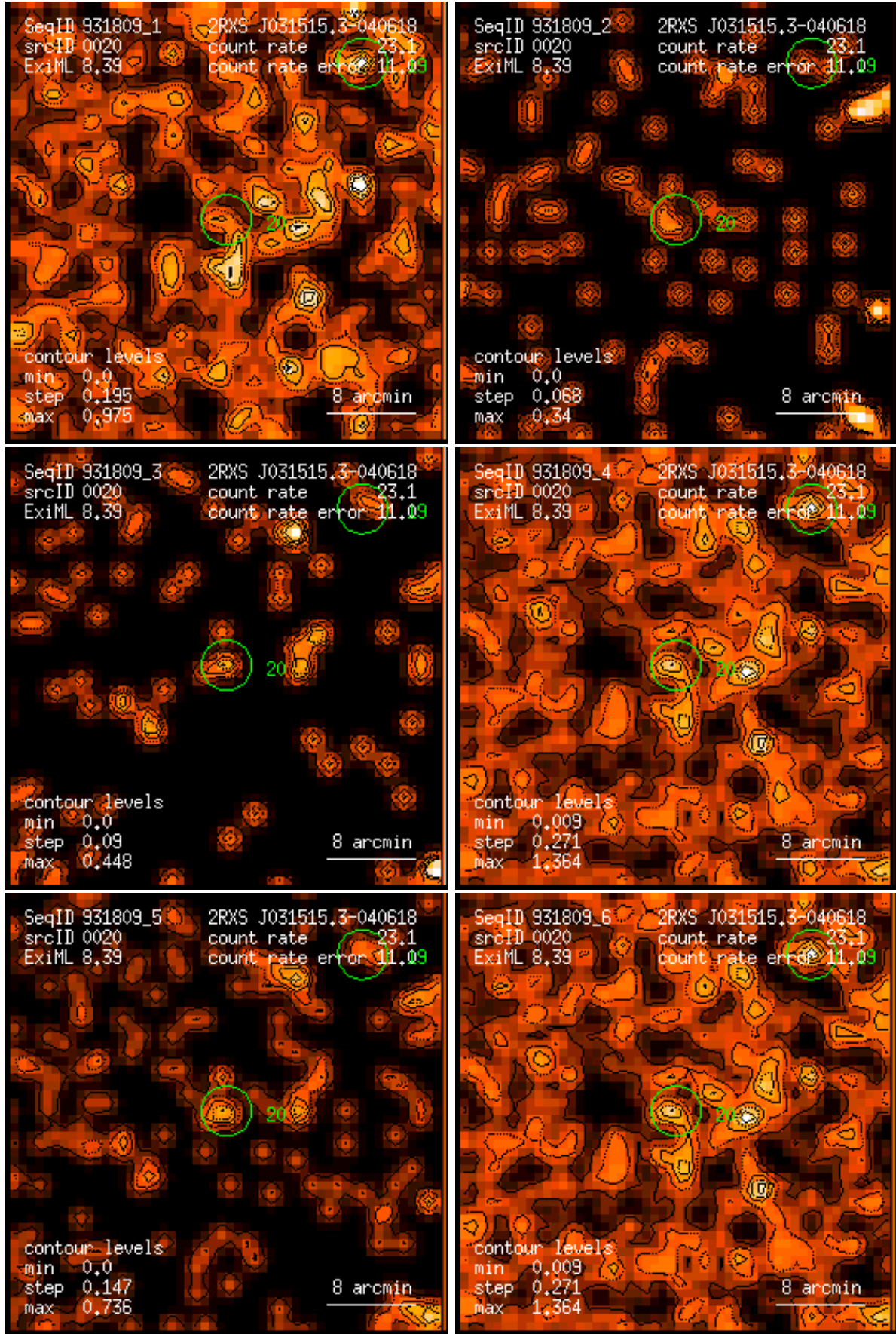
Figure 20: RASS 931809: detection 0020: band rate images, Gaussian filter: (1) PSPC channels 11 – 41, (2) 52 – 90, (3) 91 – 201, (4) 11 – 235, (5) 52 – 201, (6) 11 – 201. Broad band rates in counts/ks. Band rate contour levels in counts/ks/arcmin 2 .
