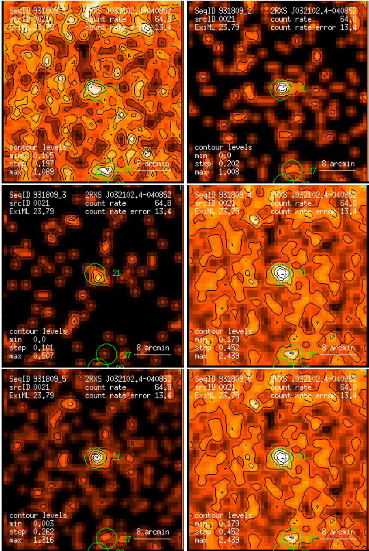
Figure 21: RASS 931809: detection 0021: band rate images, Gaussian filter: (1) PSPC channels 11 – 41, (2) 52 – 90, (3) 91 – 201, (4) 11 – 235, (5) 52 – 201, (6) 11 – 201. Broad band rates in counts/ks. Band rate contour levels in counts/ks/arcmin 2 .
