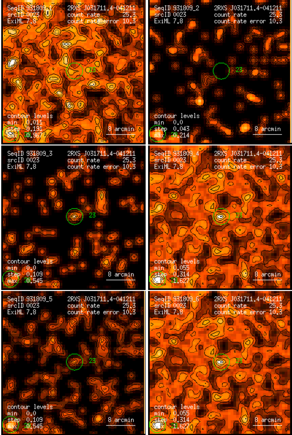
Figure 23: RASS 931809: detection 0023: band rate images, Gaussian filter: (1) PSPC channels 11 – 41, (2) 52 – 90, (3) 91 – 201, (4) 11 – 235, (5) 52 – 201, (6) 11 – 201. Broad band rates in counts/ks. Band rate contour levels in counts/ks/arcmin 2 .
