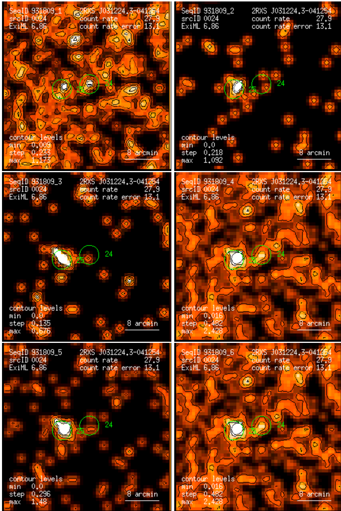
Figure 24: RASS 931809: detection 0024: band rate images, Gaussian filter: (1) PSPC channels 11 – 41, (2) 52 – 90, (3) 91 – 201, (4) 11 – 235, (5) 52 – 201, (6) 11 – 201. Broad band rates in counts/ks. Band rate contour levels in counts/ks/arcmin 2 .
