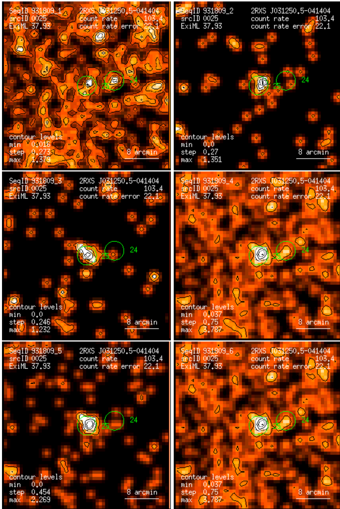
Figure 25: RASS 931809: detection 0025: band rate images, Gaussian filter: (1) PSPC channels 11 – 41, (2) 52 – 90, (3) 91 – 201, (4) 11 – 235, (5) 52 – 201, (6) 11 – 201. Broad band rates in counts/ks. Band rate contour levels in counts/ks/arcmin 2 .
