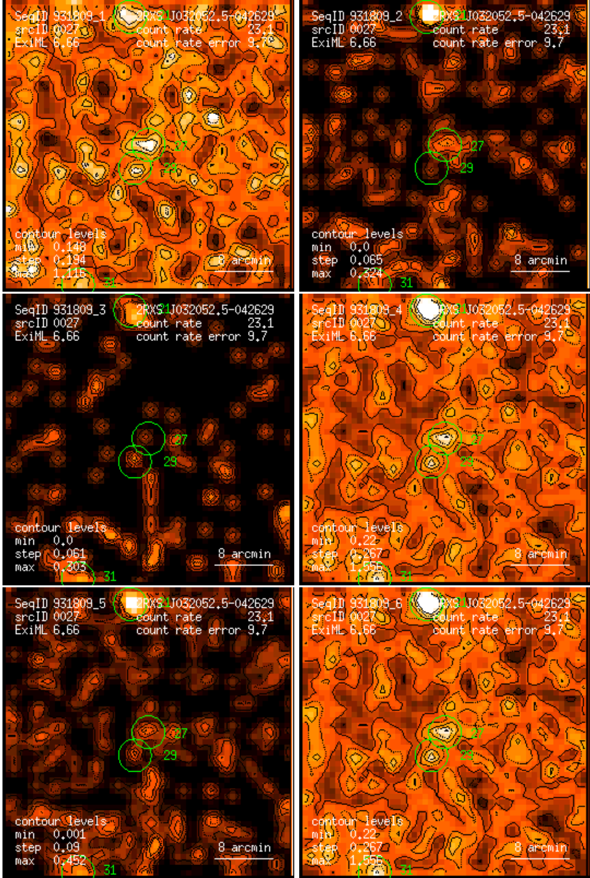
Figure 27: RASS 931809: detection 0027: band rate images, Gaussian filter: (1) PSPC channels 11 – 41, (2) 52 – 90, (3) 91 – 201, (4) 11 – 235, (5) 52 – 201, (6) 11 – 201. Broad band rates in counts/ks. Band rate contour levels in counts/ks/arcmin 2 .
