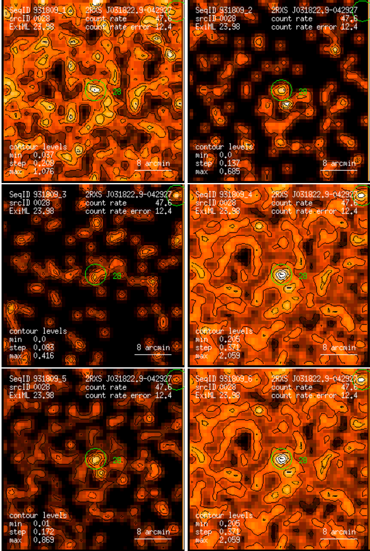
Figure 28: RASS 931809: detection 0028: band rate images, Gaussian filter: (1) PSPC channels 11 – 41, (2) 52 – 90, (3) 91 – 201, (4) 11 – 235, (5) 52 – 201, (6) 11 – 201. Broad band rates in counts/ks. Band rate contour levels in counts/ks/arcmin 2 .
