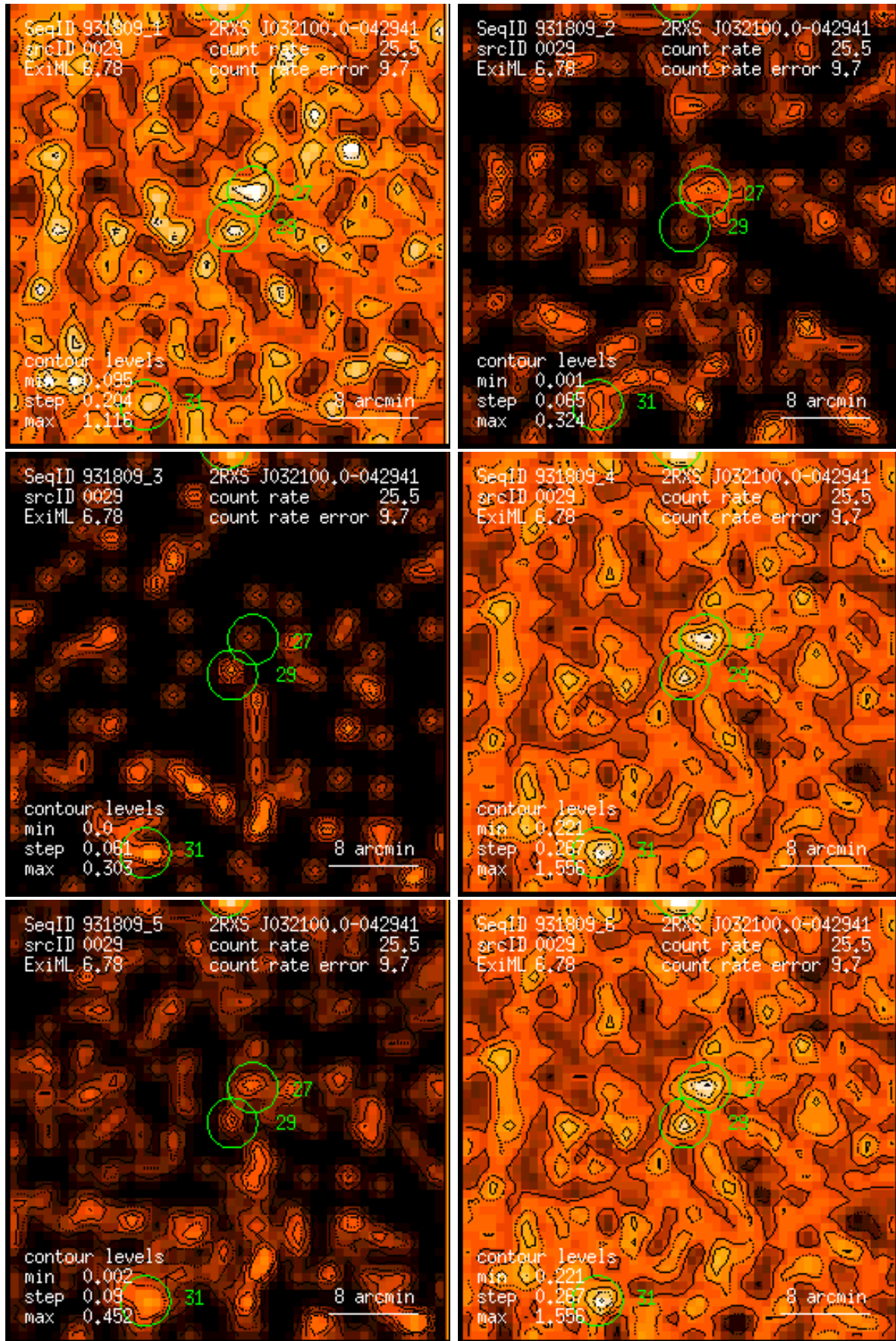
Figure 29: RASS 931809: detection 0029: band rate images, Gaussian filter: (1) PSPC channels 11 – 41, (2) 52 – 90, (3) 91 – 201, (4) 11 – 235, (5) 52 – 201, (6) 11 – 201. Broad band rates in counts/ks. Band rate contour levels in counts/ks/arcmin 2 .
