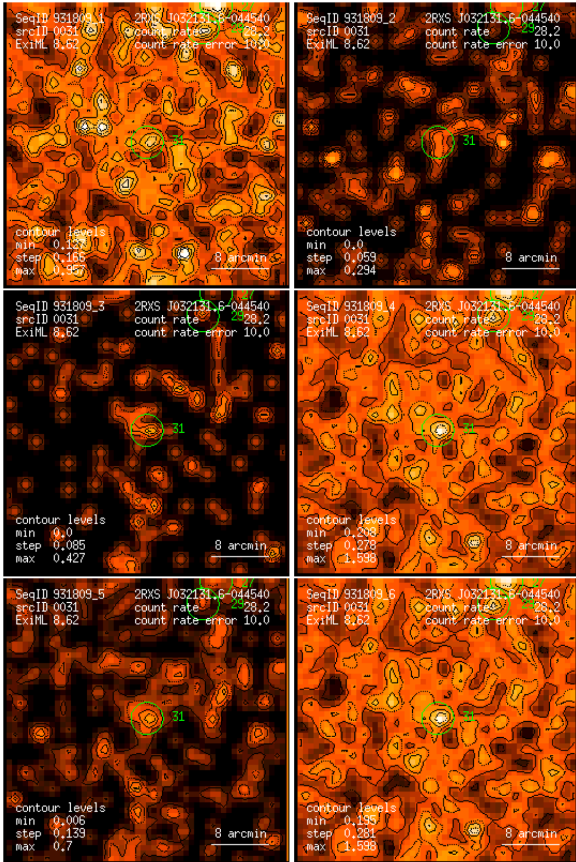
Figure 31: RASS 931809: detection 0031: band rate images, Gaussian filter: (1) PSPC channels 11 – 41, (2) 52 – 90, (3) 91 – 201, (4) 11 – 235, (5) 52 – 201, (6) 11 – 201. Broad band rates in counts/ks. Band rate contour levels in counts/ks/arcmin 2 .
