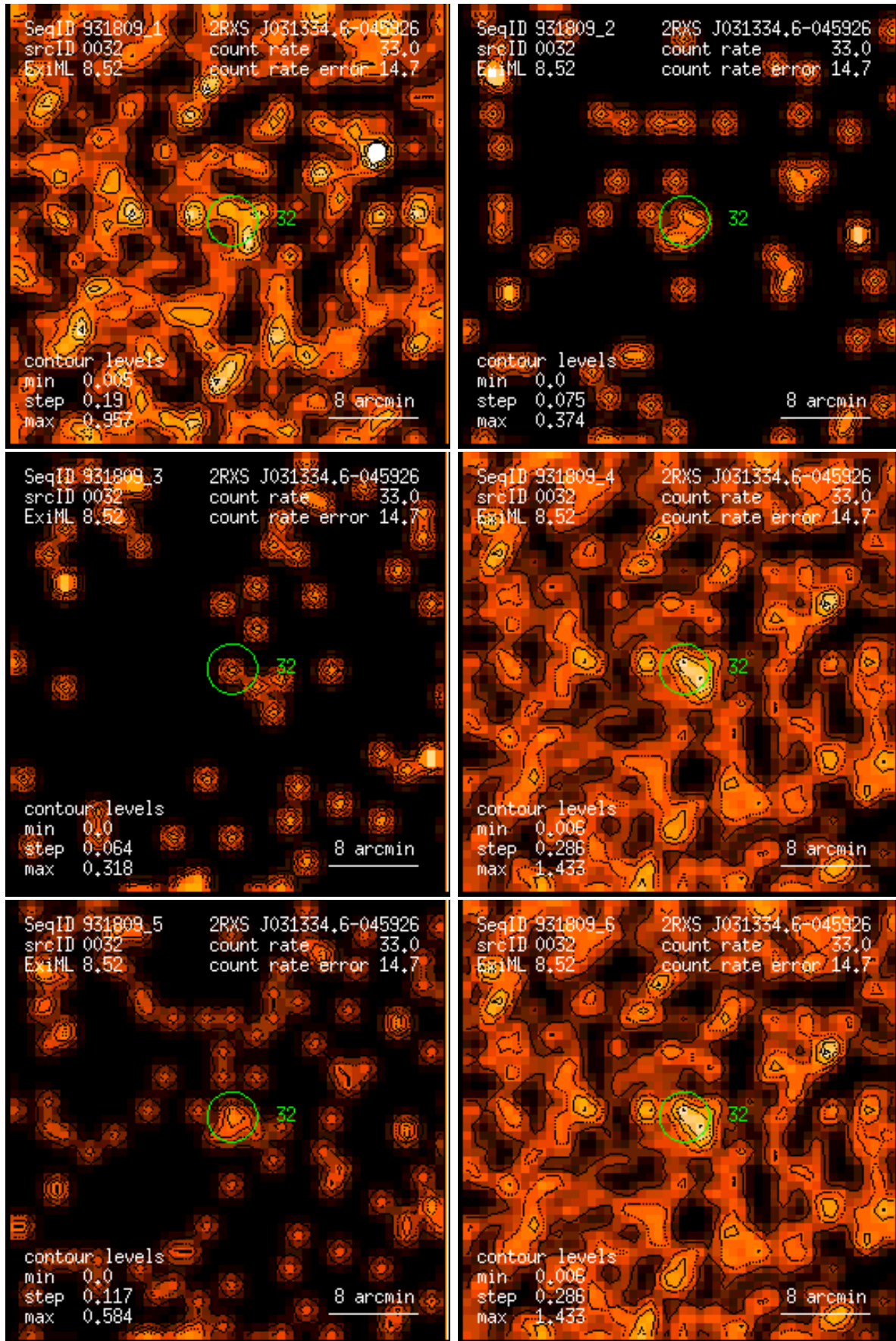
Figure 32: RASS 931809: detection 0032: band rate images, Gaussian filter: (1) PSPC channels 11 – 41, (2) 52 – 90, (3) 91 – 201, (4) 11 – 235, (5) 52 – 201, (6) 11 – 201. Broad band rates in counts/ks. Band rate contour levels in counts/ks/arcmin 2 .
