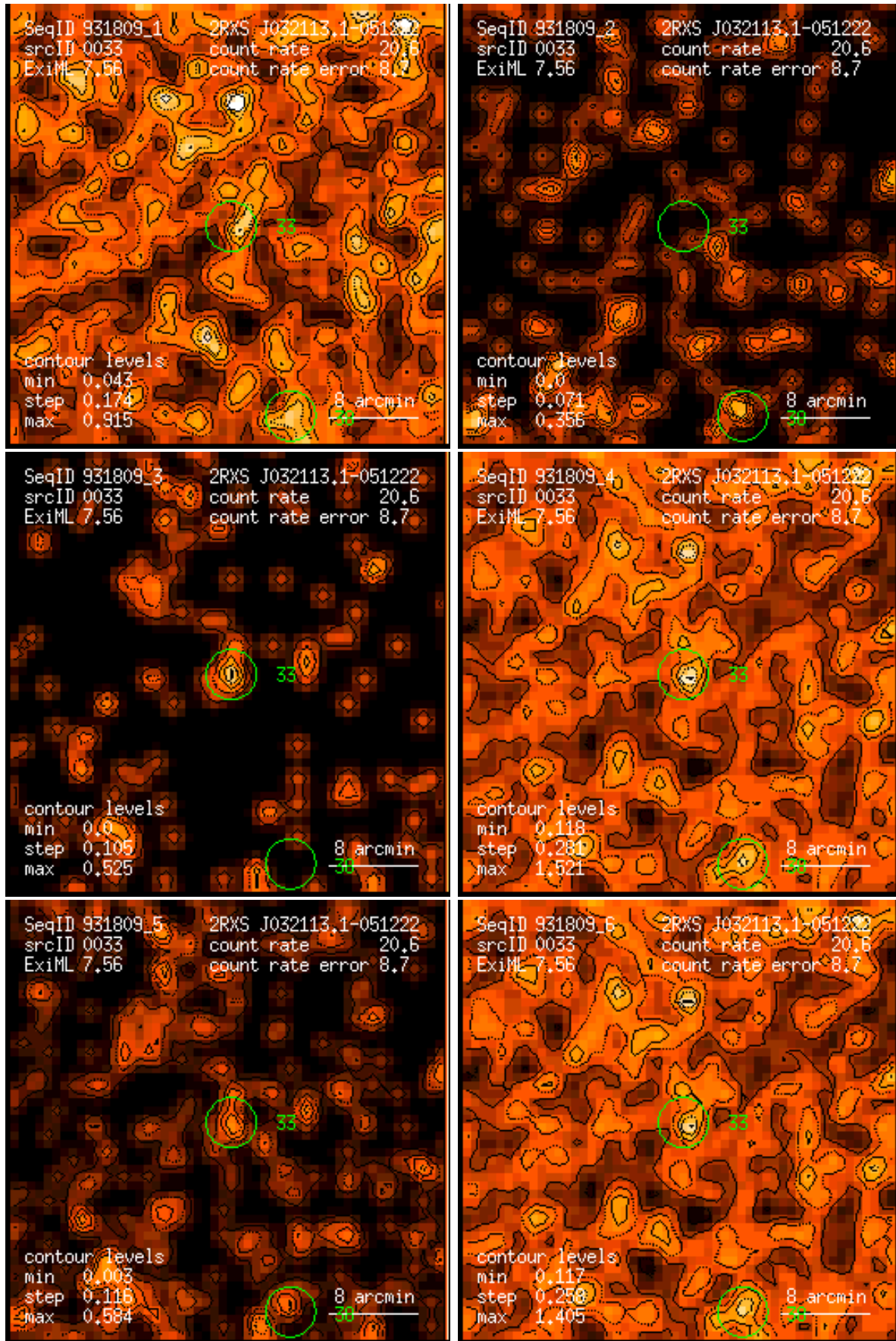
Figure 33: RASS 931809: detection 0033: band rate images, Gaussian filter: (1) PSPC channels 11 – 41, (2) 52 – 90, (3) 91 – 201, (4) 11 – 235, (5) 52 – 201, (6) 11 – 201. Broad band rates in counts/ks. Band rate contour levels in counts/ks/arcmin 2 .
