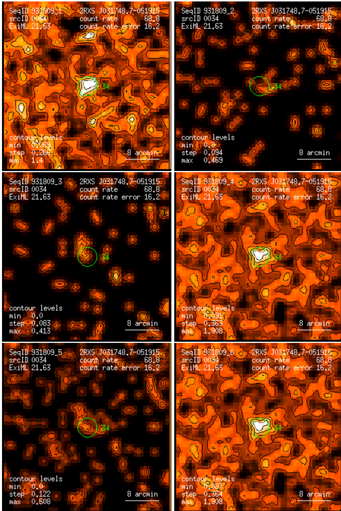
Figure 34: RASS 931809: detection 0034: band rate images, Gaussian filter: (1) PSPC channels 11 – 41, (2) 52 – 90, (3) 91 – 201, (4) 11 – 235, (5) 52 – 201, (6) 11 – 201. Broad band rates in counts/ks. Band rate contour levels in counts/ks/arcmin 2 .
