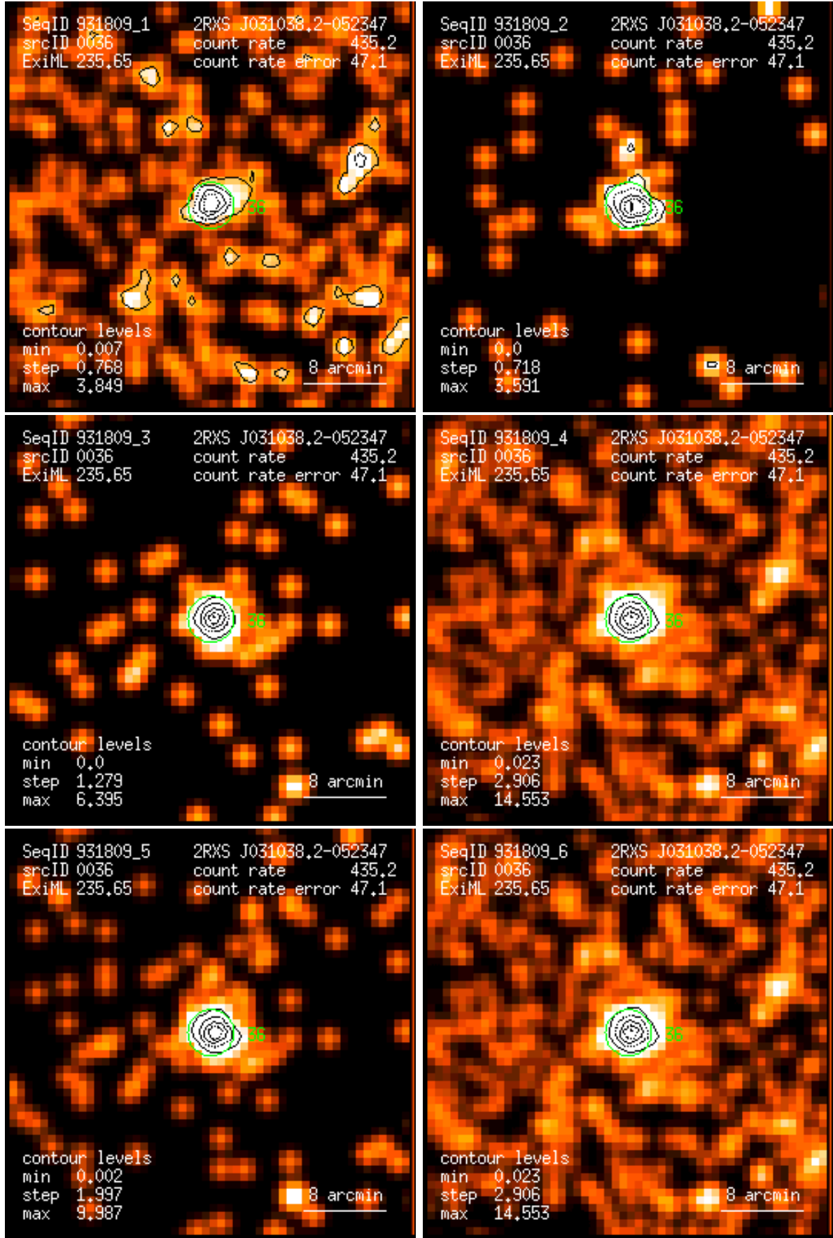
Figure 36: RASS 931809: detection 0036: band rate images, Gaussian filter: (1) PSPC channels 11 – 41, (2) 52 – 90, (3) 91 – 201, (4) 11 – 235, (5) 52 – 201, (6) 11 – 201. Broad band rates in counts/ks. Band rate contour levels in counts/ks/arcmin 2 .
