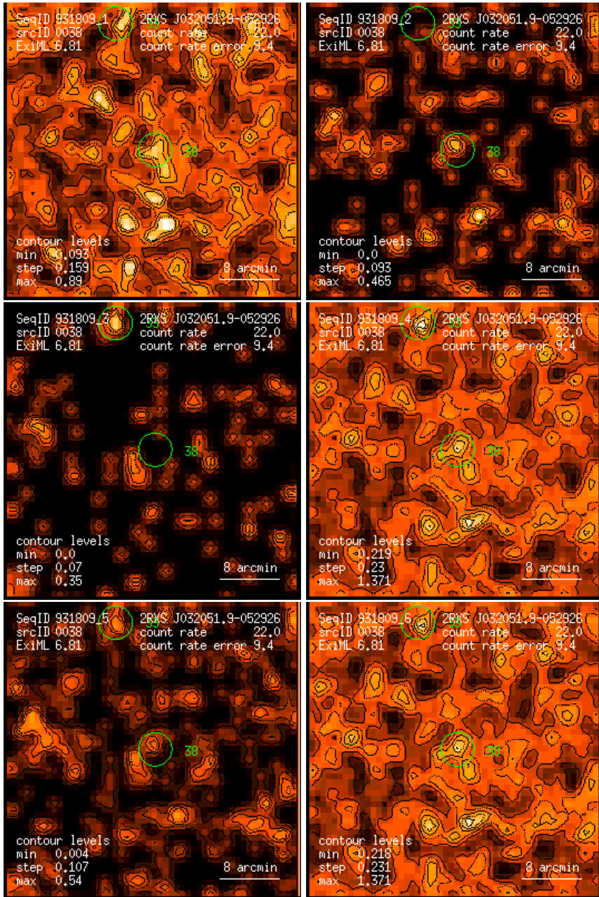
Figure 38: RASS 931809: detection 0038: band rate images, Gaussian filter: (1) PSPC channels 11 – 41, (2) 52 – 90, (3) 91 – 201, (4) 11 – 235, (5) 52 – 201, (6) 11 – 201. Broad band rates in counts/ks. Band rate contour levels in counts/ks/arcmin 2 .
