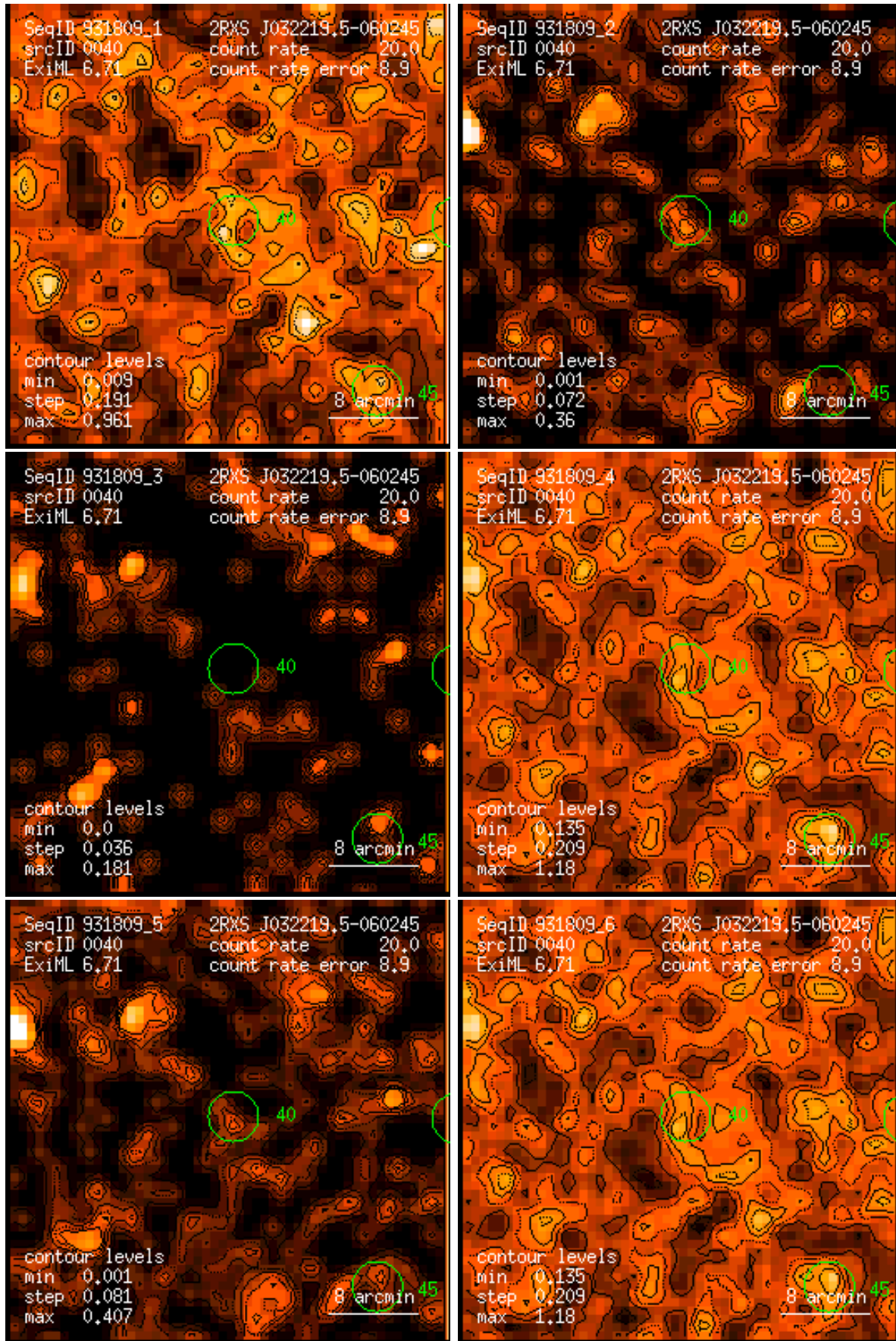
Figure 40: RASS 931809: detection 0040: band rate images, Gaussian filter: (1) PSPC channels 11 – 41, (2) 52 – 90, (3) 91 – 201, (4) 11 – 235, (5) 52 – 201, (6) 11 – 201. Broad band rates in counts/ks. Band rate contour levels in counts/ks/arcmin 2 .
