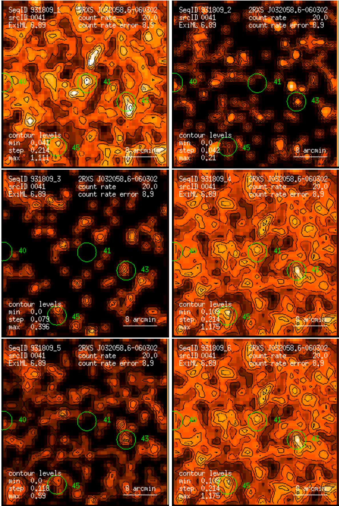
Figure 41: RASS 931809: detection 0041: band rate images, Gaussian filter: (1) PSPC channels 11 – 41, (2) 52 – 90, (3) 91 – 201, (4) 11 – 235, (5) 52 – 201, (6) 11 – 201. Broad band rates in counts/ks. Band rate contour levels in counts/ks/arcmin 2 .
