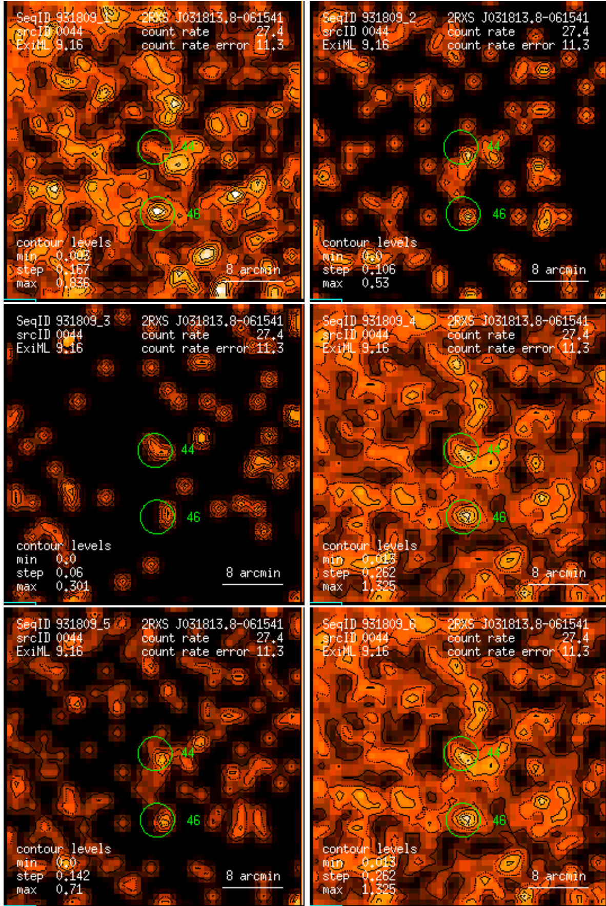
Figure 44: RASS 931809: detection 0044: band rate images, Gaussian filter: (1) PSPC channels 11 – 41, (2) 52 – 90, (3) 91 – 201, (4) 11 – 235, (5) 52 – 201, (6) 11 – 201. Broad band rates in counts/ks. Band rate contour levels in counts/ks/arcmin 2 .
