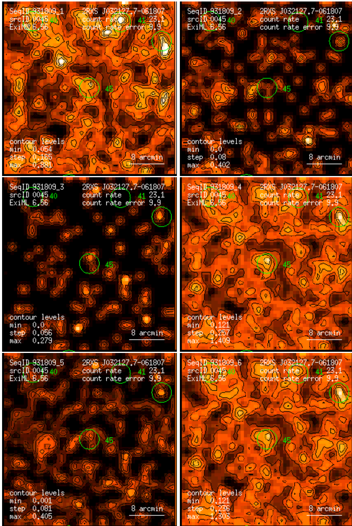
Figure 45: RASS 931809: detection 0045: band rate images, Gaussian filter: (1) PSPC channels 11 – 41, (2) 52 – 90, (3) 91 – 201, (4) 11 – 235, (5) 52 – 201, (6) 11 – 201. Broad band rates in counts/ks. Band rate contour levels in counts/ks/arcmin 2 .
