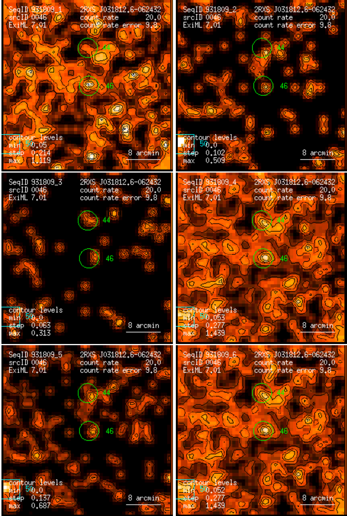
Figure 46: RASS 931809: detection 0046: band rate images, Gaussian filter: (1) PSPC channels 11 – 41, (2) 52 – 90, (3) 91 – 201, (4) 11 – 235, (5) 52 – 201, (6) 11 – 201. Broad band rates in counts/ks. Band rate contour levels in counts/ks/arcmin 2 .
