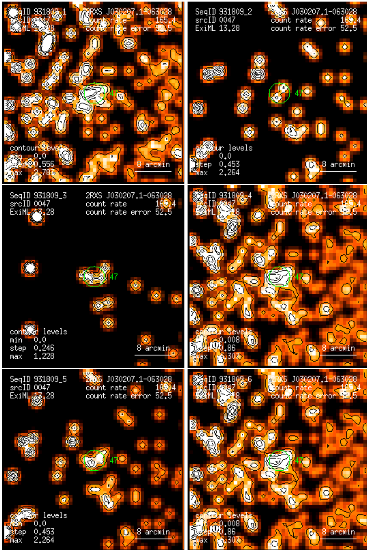
Figure 47: RASS 931809: detection 0047: band rate images, Gaussian filter: (1) PSPC channels 11 – 41, (2) 52 – 90, (3) 91 – 201, (4) 11 – 235, (5) 52 – 201, (6) 11 – 201. Broad band rates in counts/ks. Band rate contour levels in counts/ks/arcmin 2 .
