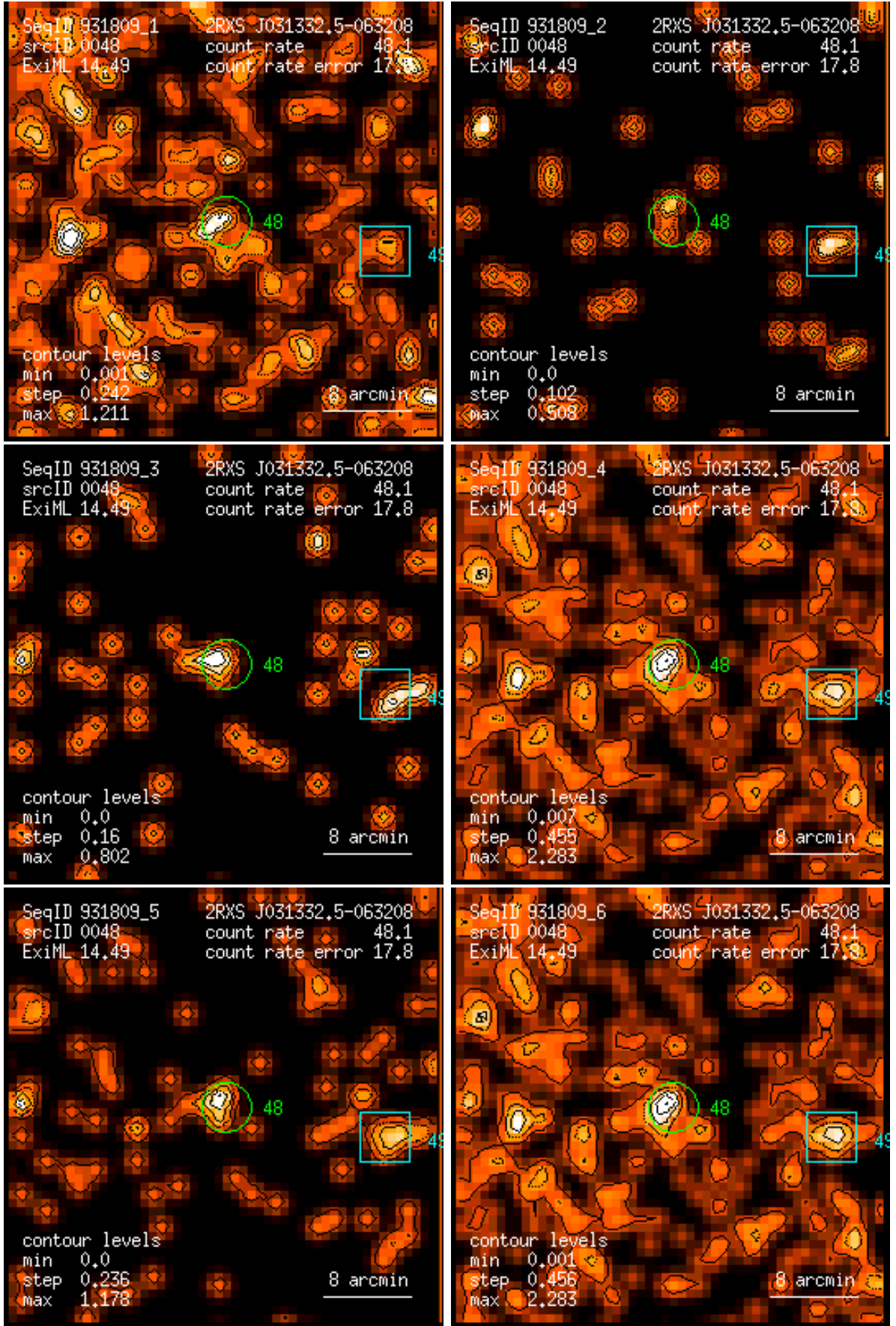
Figure 48: RASS 931809: detection 0048: band rate images, Gaussian filter: (1) PSPC channels 11 – 41, (2) 52 – 90, (3) 91 – 201, (4) 11 – 235, (5) 52 – 201, (6) 11 – 201. Broad band rates in counts/ks. Band rate contour levels in counts/ks/arcmin 2 .
