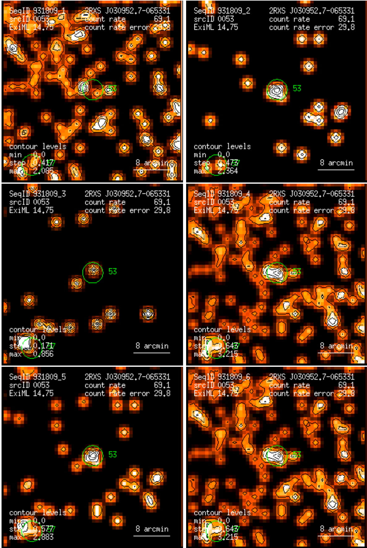
Figure 53: RASS 931809: detection 0053: band rate images, Gaussian filter: (1) PSPC channels 11 – 41, (2) 52 – 90, (3) 91 – 201, (4) 11 – 235, (5) 52 – 201, (6) 11 – 201. Broad band rates in counts/ks. Band rate contour levels in counts/ks/arcmin 2 .
